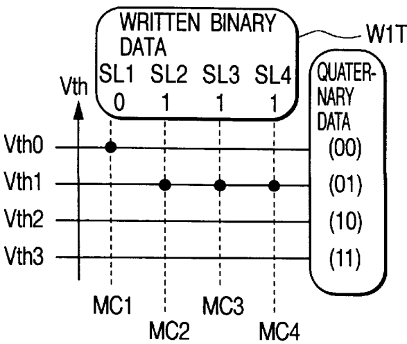
FIG. 67 CHANGE IN THRESHOLD VOLTAGE OF MEMORY CELL AT "WRITE 1"
