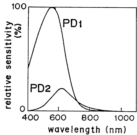
PRIOR ART Fig. 3
