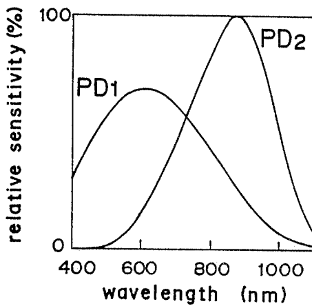
PRIOR ART Fig. 2
