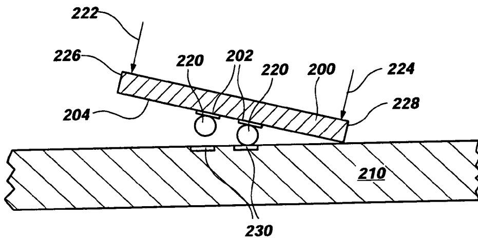
Fig. 3 (PRIOR ART)
