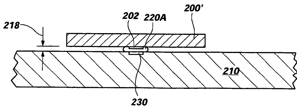
Fig. 7 (PRIOR ART)
