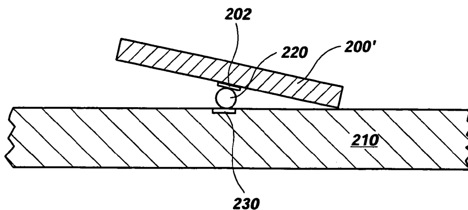
Fig. 5 (PRIOR ART)
