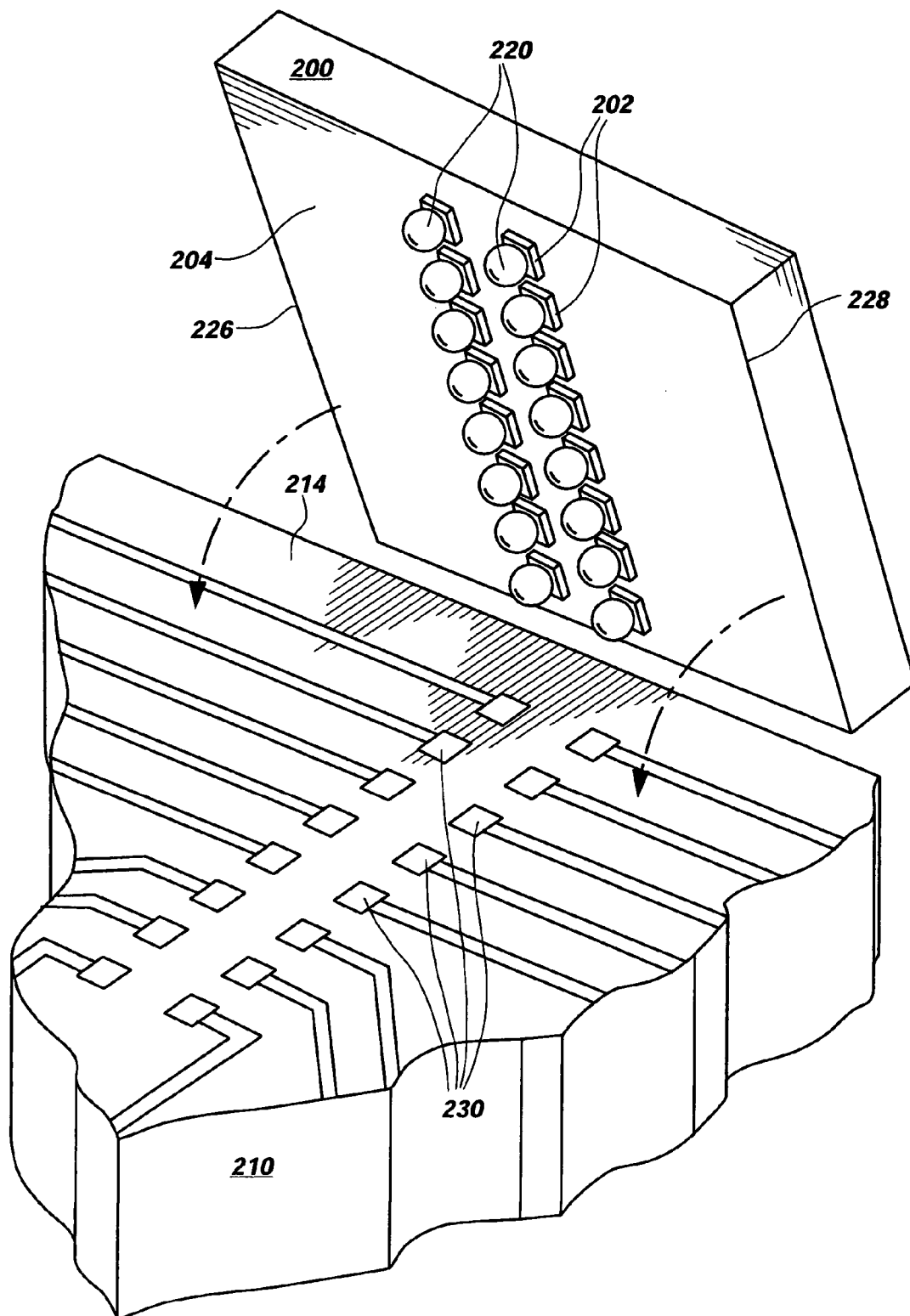
Fig. 1 (PRIOR ART)
