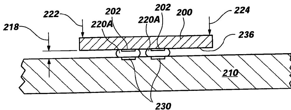
Fig. 4 (PRIOR ART)
