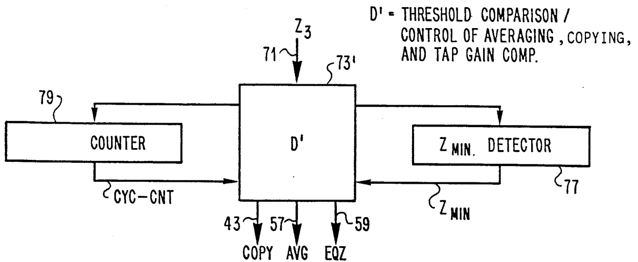
FIG. 5 ALTERNATIVE EVALUATION AND CONTROL MEANS
