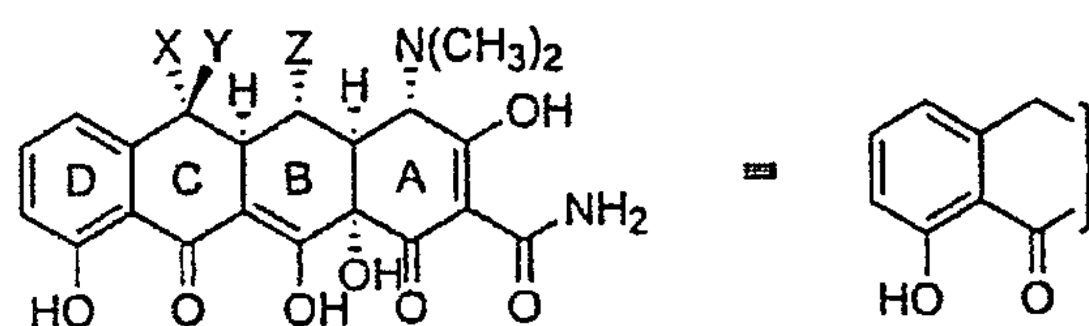
Figure 14A Representative Structures
