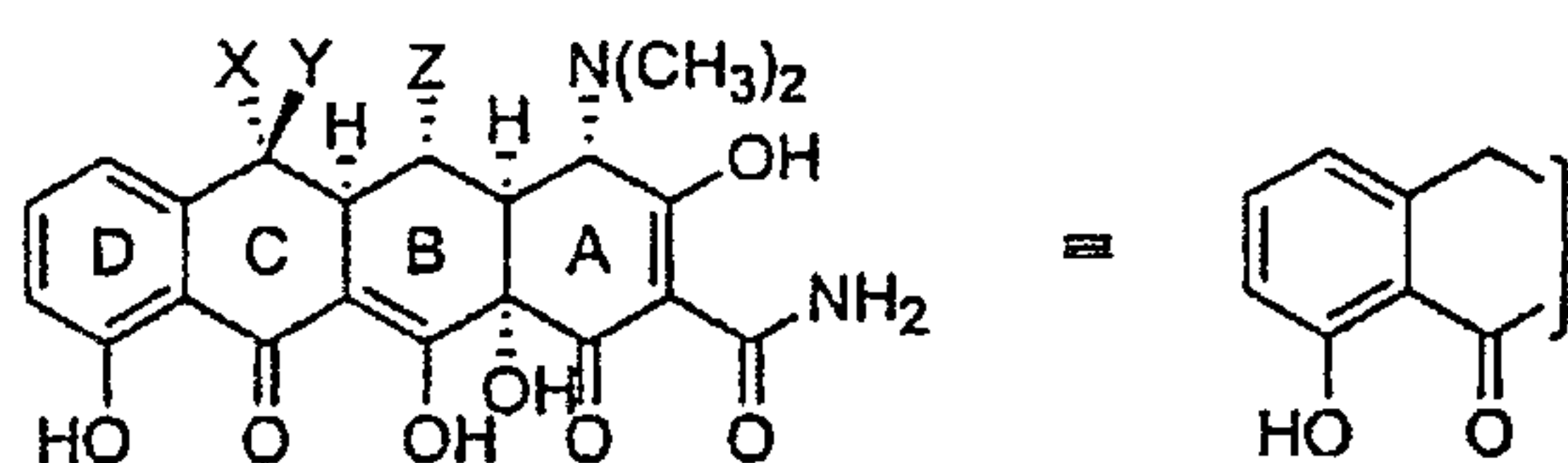
Figure 14B Representative Structures
