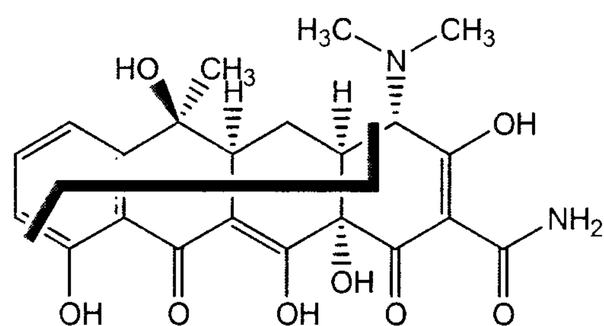
Tetracycline (3)
