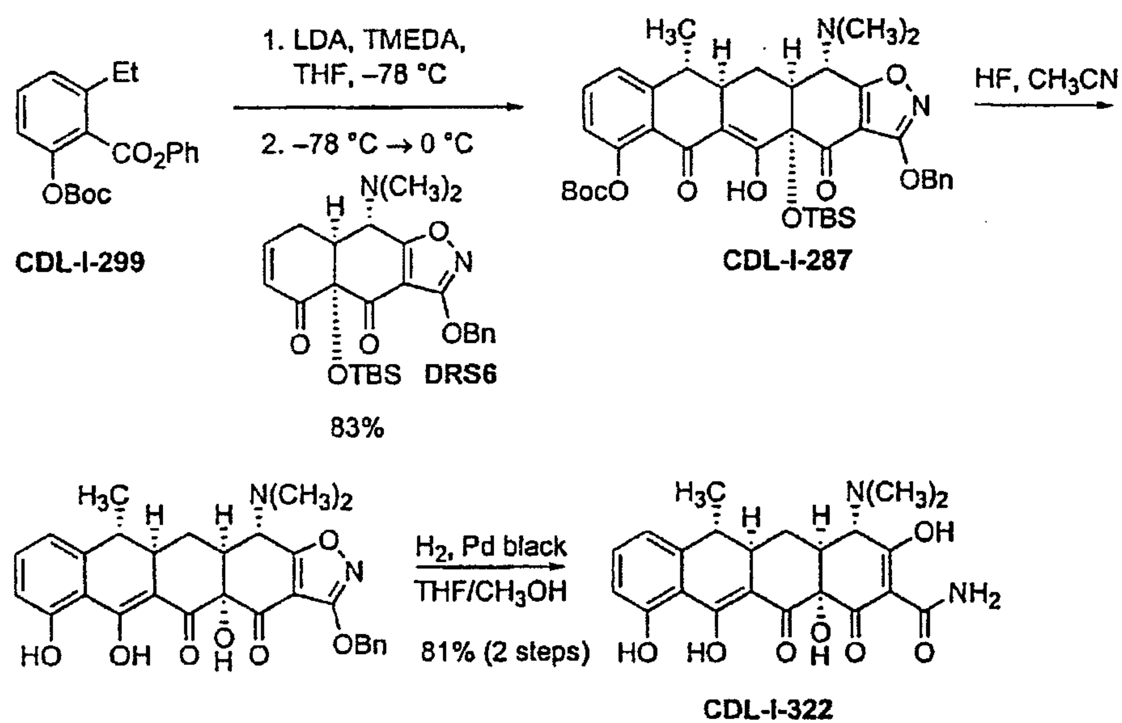
Figure 12 Total Synthesis of 6-Deoxytetracycline
