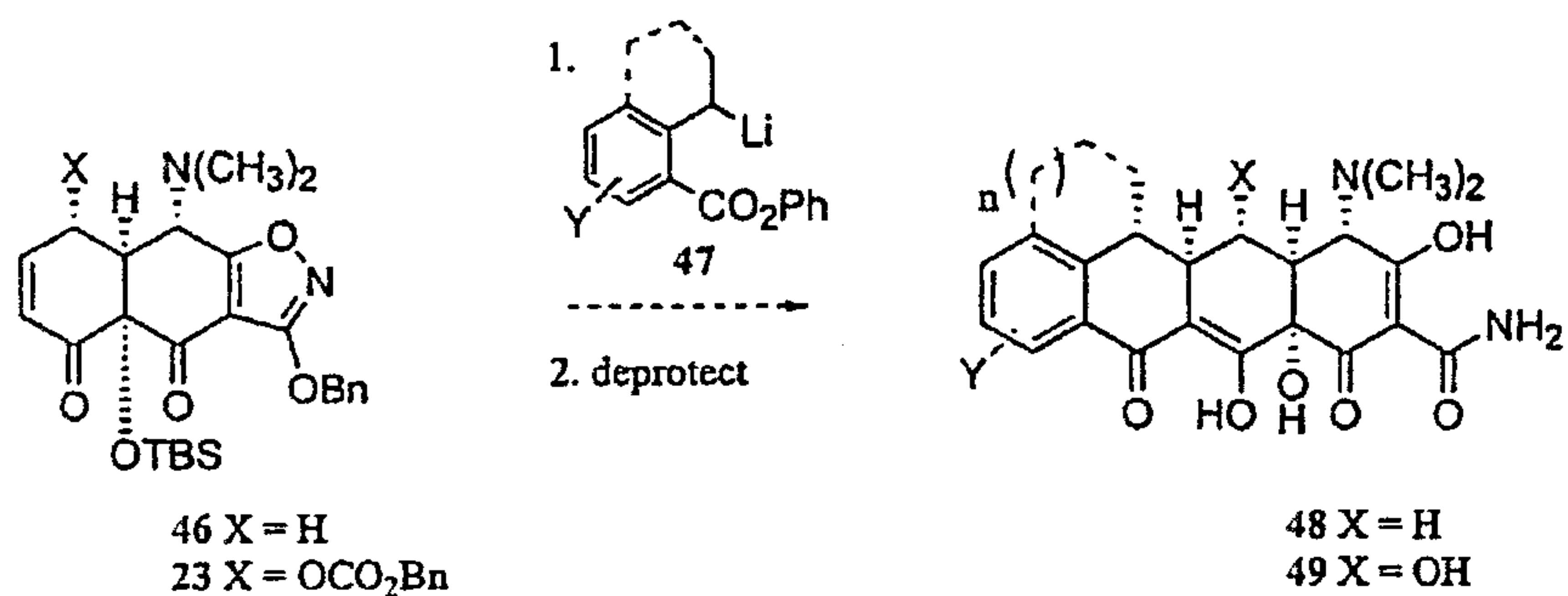
Figure 9 Summary of Targeted "Bridged-Pentacyclines"
