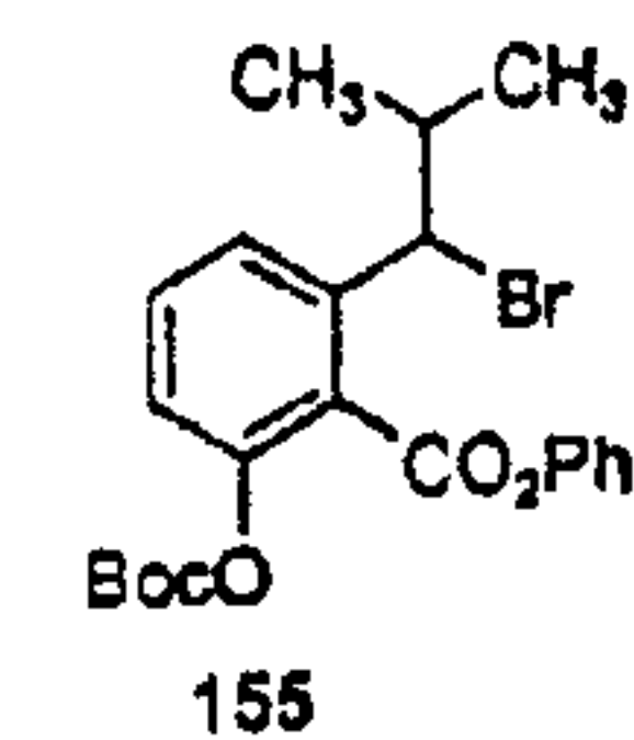
D-Ring Precursor
