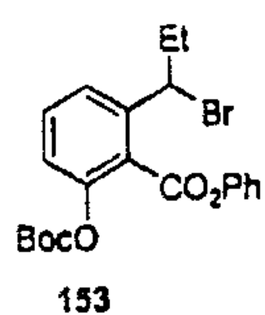
D-Ring Precursor
