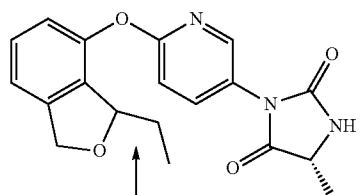
chiral-diastereoisomers 1
