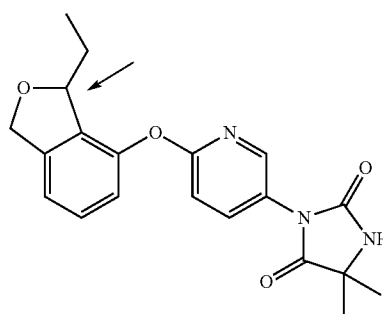
racemic mixture
