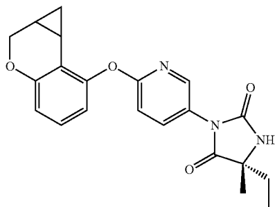
diastereoisomer 1
