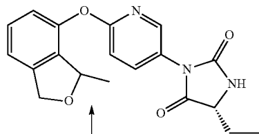
chiral-diastereoisomers 1
