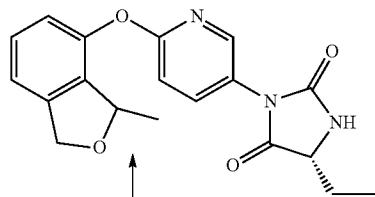
chiral-diastereoisomers 2
