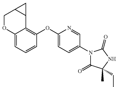
diastereoisomer 2
