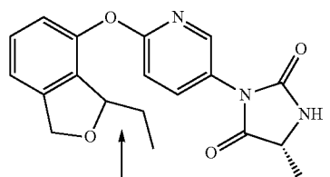
2 diastereoisomers
