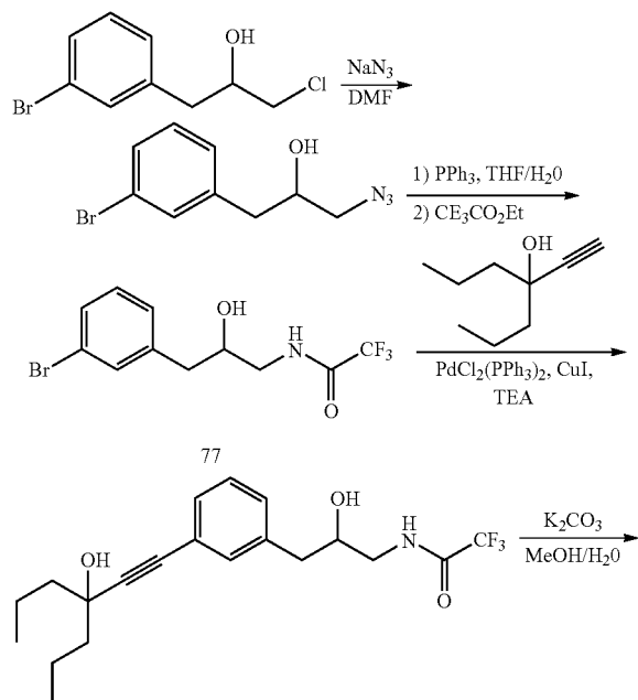
SCHEME 19
