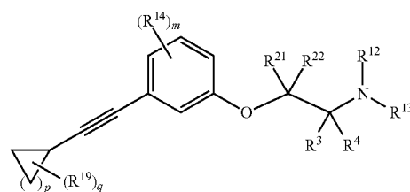
Formula (G)
