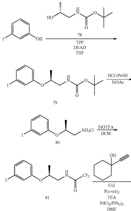
SCHEME 20
