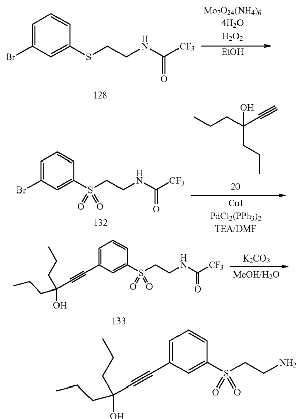
SCHEME 32
