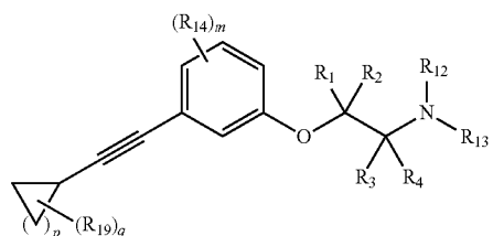
Formula (IIIb)
