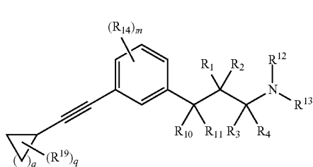
Formula (IIc)
