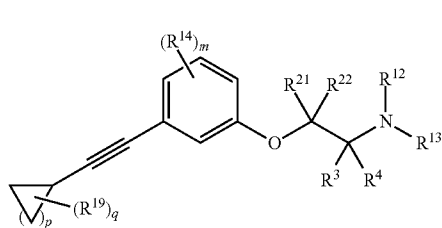
Formula (G)
