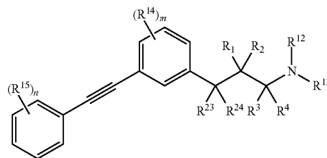
Formula (C)
