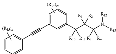
Formula (IIb)
