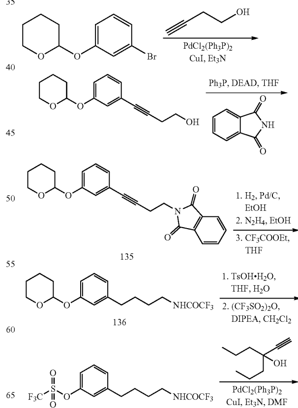
SCHEME 33
