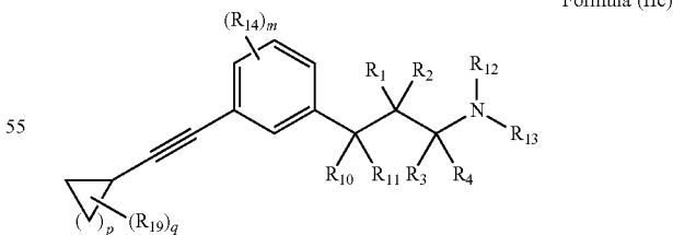
Formula (IIc)
