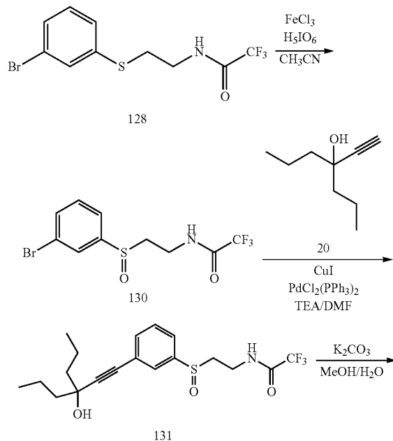
SCHEME 31
