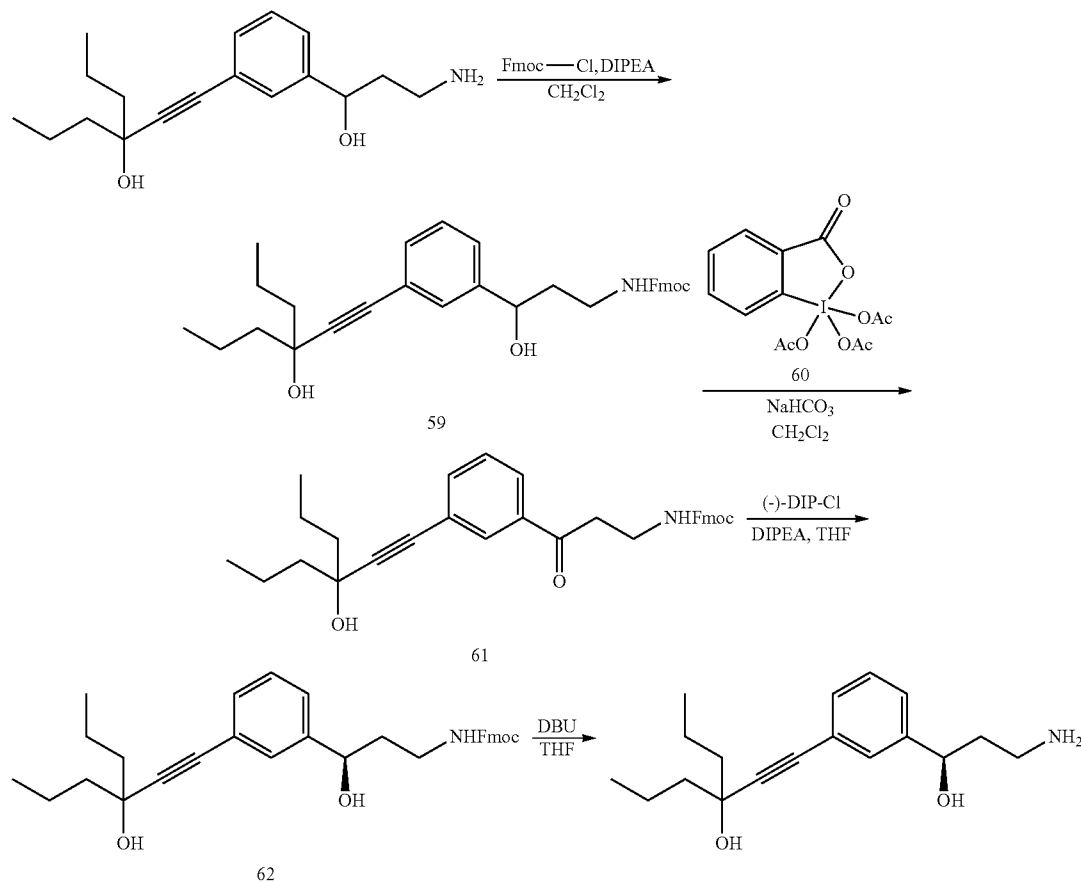
Scheme 15
