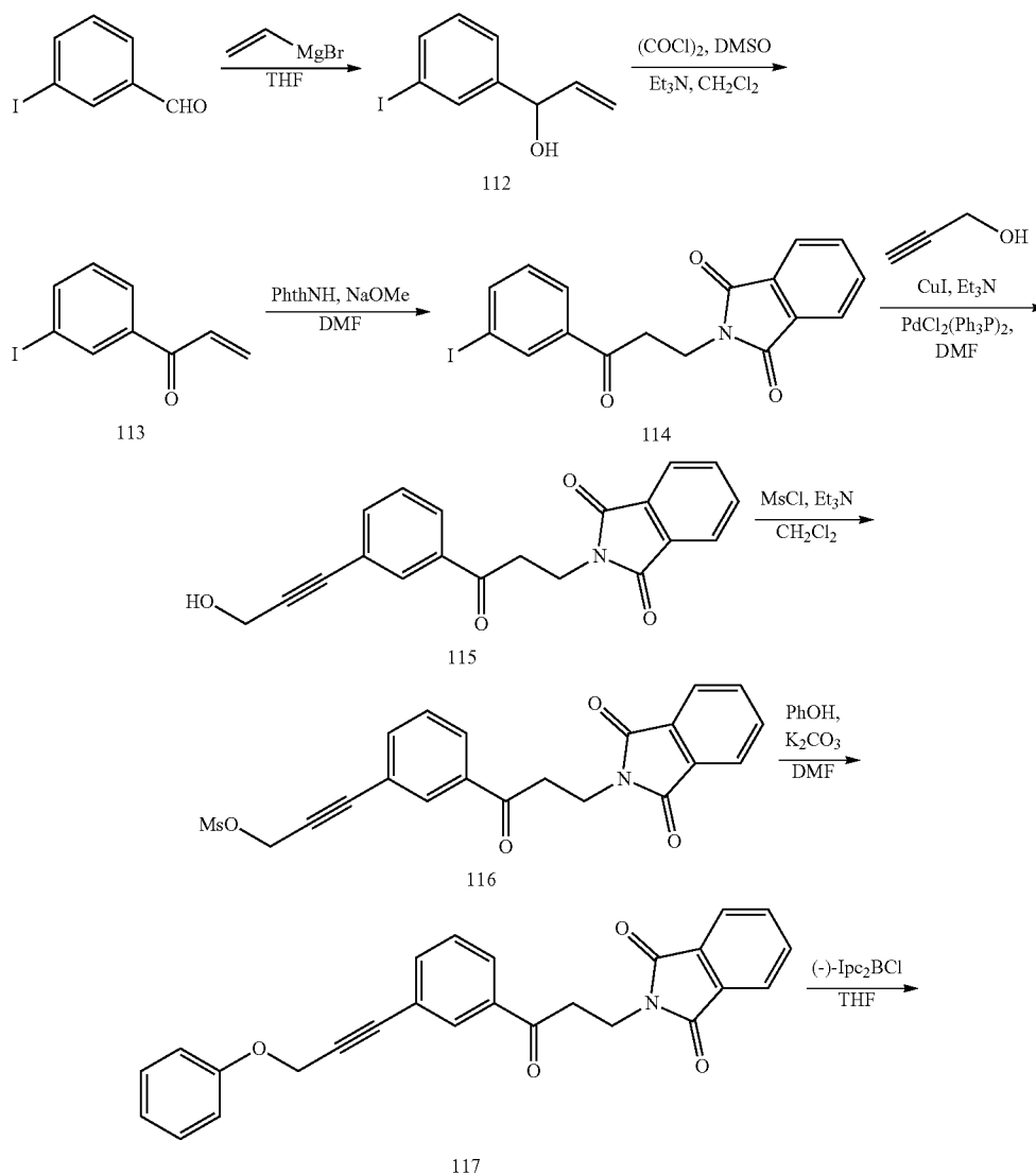
SCHEME 28
