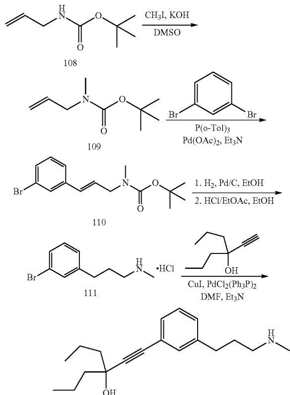
SCHEME 27
