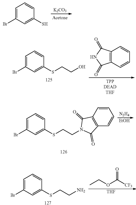
SCHEME 30
