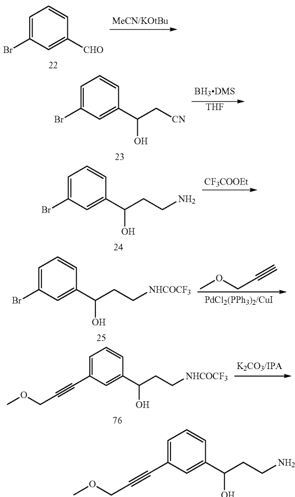
SCHEME 18
