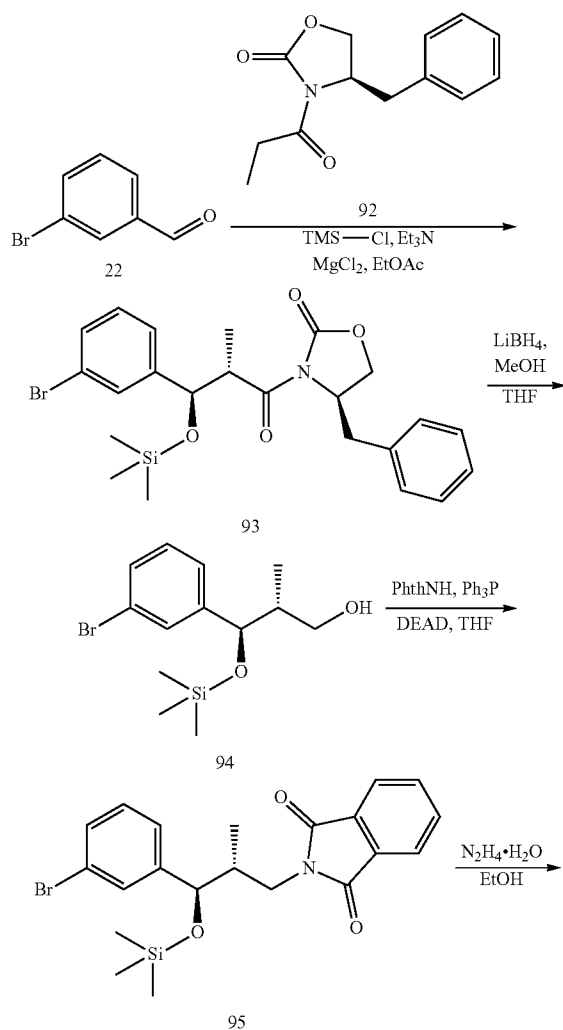
SCHEME 24
