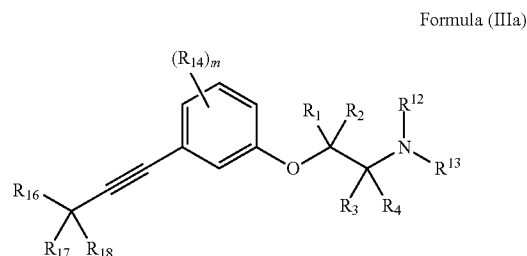
Formula (IIIa)
