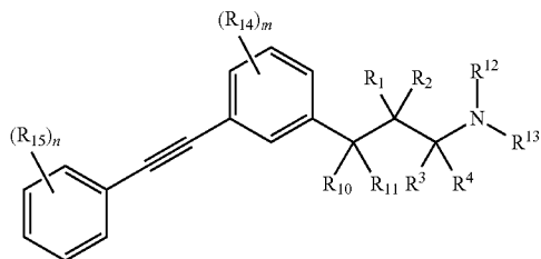
Formula (IIa)
