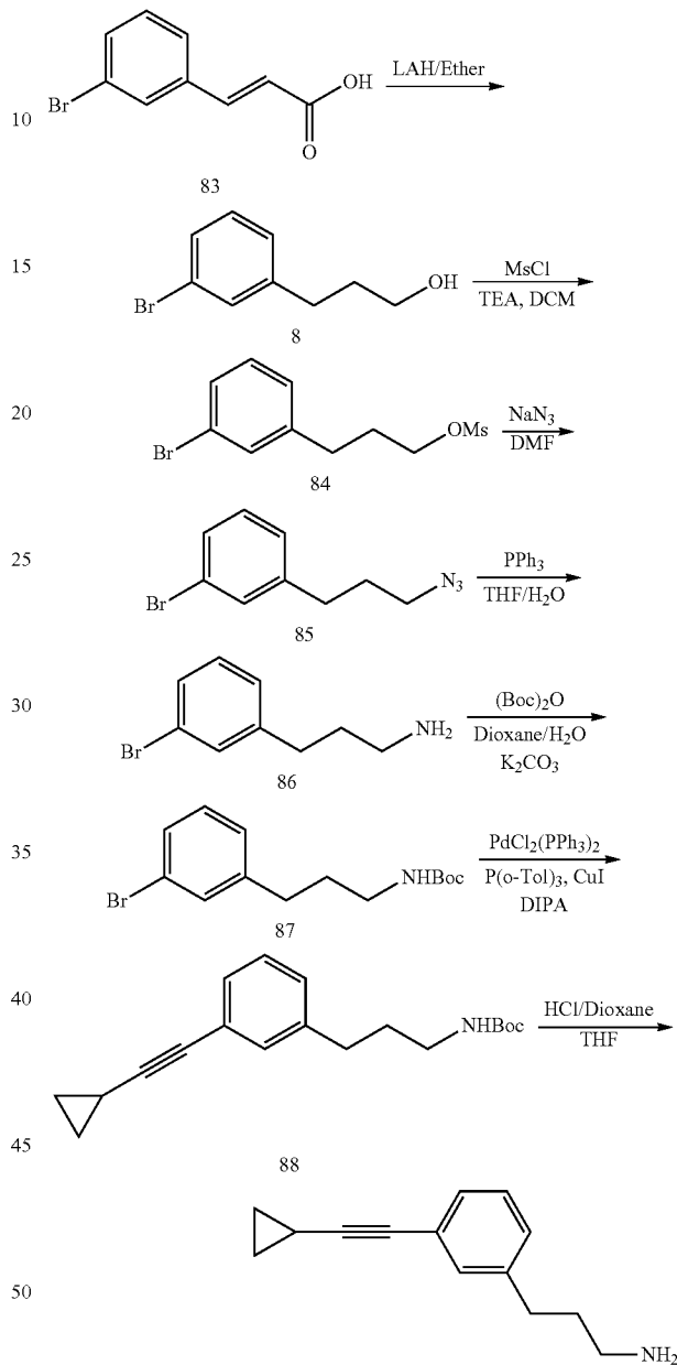
SCHEME 21
