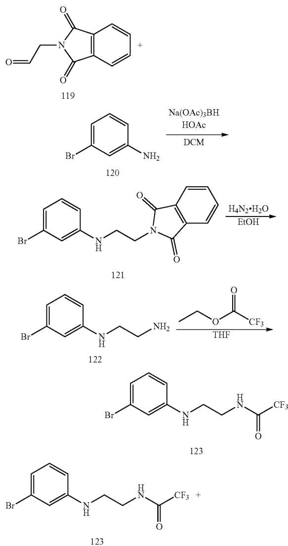
SCHEME 29
