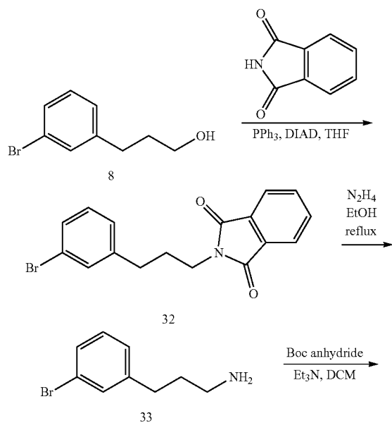
SCHEME 7
