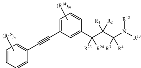
Formula (B)
