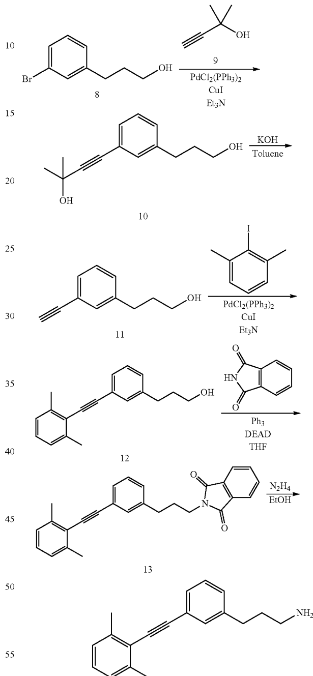
SCHEME 3
