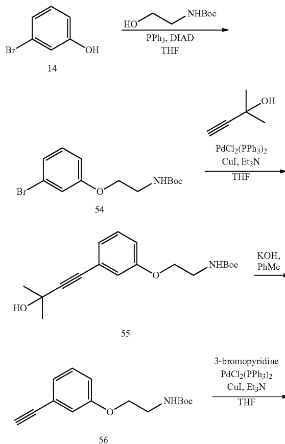
SCHEME 13
