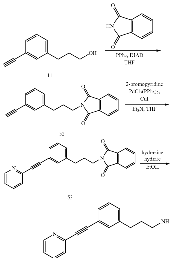
SCHEME 12
