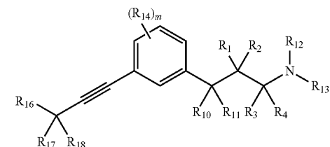
Formula (IIc)
