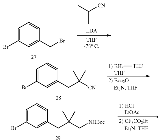
SCHEME 6
