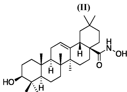
(3 \beta ) 3-Hydroxy-N-hydroxy-olean-12-en-28-amide
