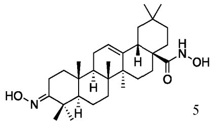
3-hydroxyimino-N-hydroxy-oléan-12-ène-28-amide
