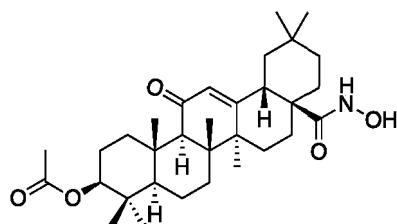
(3 \beta ) 3-Acetyloxy-11-oxo-olean-12-en-N-hydroxy-28-amide
