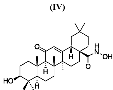
(3 \beta ) 3-Hydroxy-11-oxo-olean-12-en-N-hydroxy-28-amide
