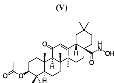
(3β) 3-Acetyloxy-11-oxo-olean-12-en-N-hydroxy-28-amide
