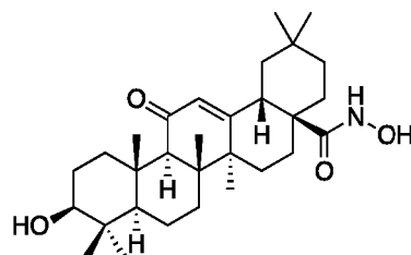
(3β)-3-Hydroxy-11-oxoolean-12-en-N-hydroxy-28-amid
