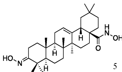
3-Hydroxyimino-N-hydroxyolean-12-en-28-amid
