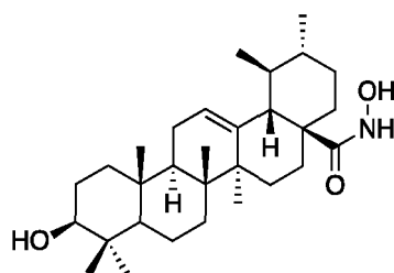
(3 \beta ) 3-hydroxy-N-hydroxy-urs-12-ène-28-amide
