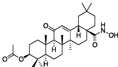
(3 \beta ) 3-Acetyloxy-11-oxo-olean-12-en-N-hydroxy-28-amide;
