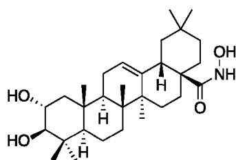
(2α,3β)2,3-dihydroxy-N-hydroxy-oléan-12-ène-28-amide
