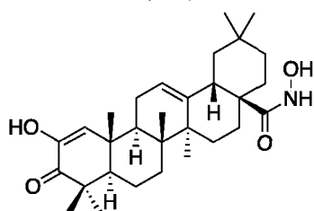
2-Hydroxy-3-oxo-oleana-1,12-dien-N-hydroxy-28-amide.
