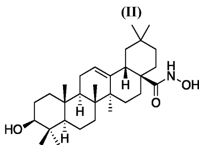
(3β)-3-Hydroxy-N-hydroxyolean-12-en-28-amid
