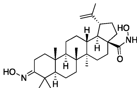
3-hydroxyimino-N-hydroxy-lup-20(29)-en-28-amide
