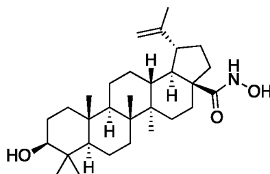
(3 \beta ) 3-hydroxy-N-hydroxy-lup-20(29)-ène-28-amide
