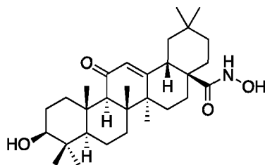
(3 \beta ) 3-Hydroxy-11-oxo-olean-12-en-N-hydroxy-28-amide
