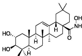
(2α,3β) 2,3-Dihydroxy-N-hydroxy-olean-12-en-28-amide
