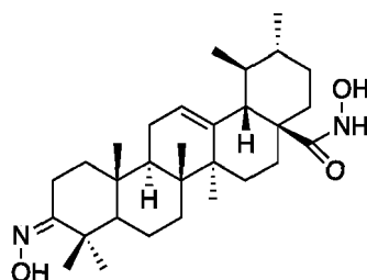
3-hydroxyimino-N-hydroxy-urs-12-ène-28-amide
