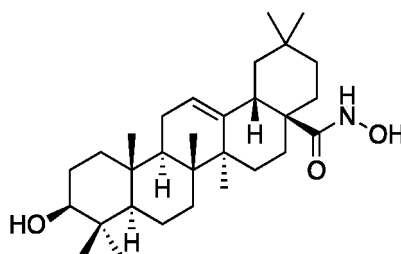
(3β)-3-Hydroxy-N-hydroxyolean-12-en-28-amid
