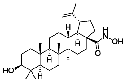
(3 \beta ) 3-Hydroxy-N-hydroxy-lup-20(29)-en-28-amide
