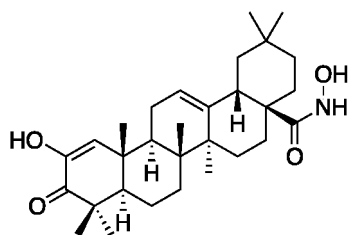
2-Hydroxy-3-oxo-oléan-1,12-diène-N-hydroxy-28-amide
