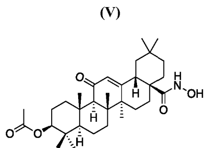
(3 \beta ) 3-Acetyloxy-11-oxo-olean-12-en-N-hydroxy-28-amide
