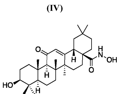
(3β) 3-Hydroxy-11-oxo-olean-12-en-N-hydroxy-28-amide
