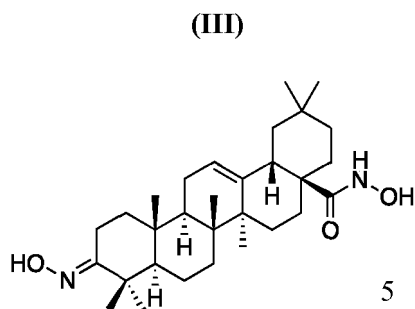
3-Hydroxyimino-N-hydroxy-olean-12-en-28-amide
