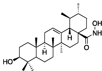
(3β) 3-hydroxy-N-hydroxy-urs-12-ène-28-amide
