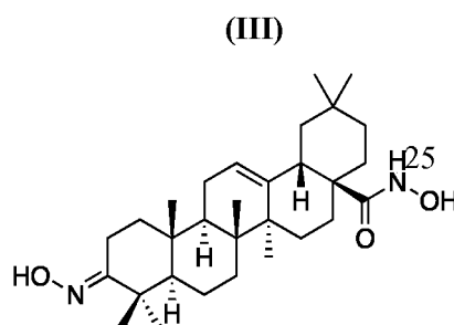
3-Hydroxyimino-N-hydroxy-olean-12-en-28-amide
