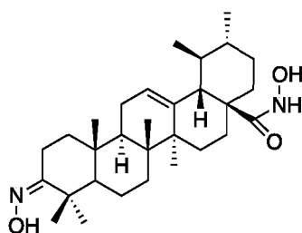
3-Hydroxyimino-N-hydroxy-urs-12-en-28-amide
