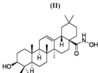
(3β) 3-Hydroxy-N-hydroxy-olean-12-en-28-amide
