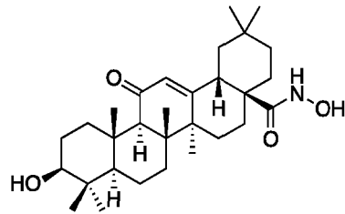
(3β) 3-hydroxy-11-oxo-oléan-12-ène-N-hydroxy-28-amide ;
