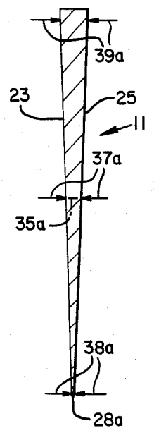
FIG. 3 (PRIOR ART)
