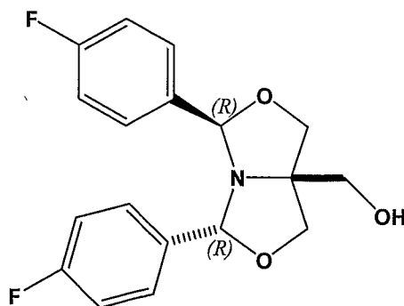
R/R isomer GS-164 (Shintani 1997)
