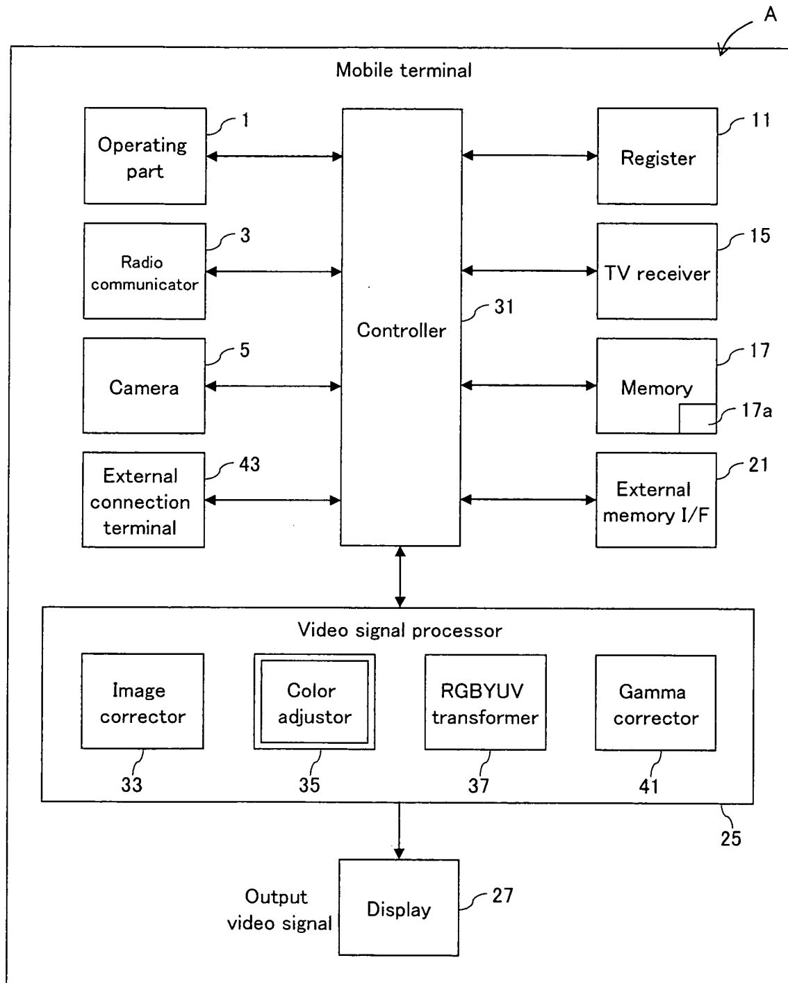
Configuration example of mobile terminal
