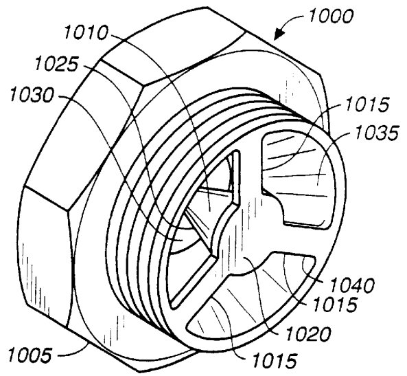
FIG. 10 (PRIOR ART)
