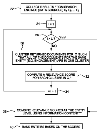
ALGORITHM OF MERGING SEARCH RESULTS
