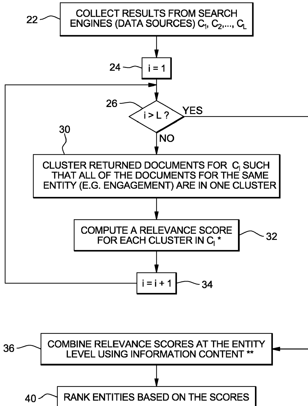
ALGORITHM OF MERGING SEARCH RESULTS
