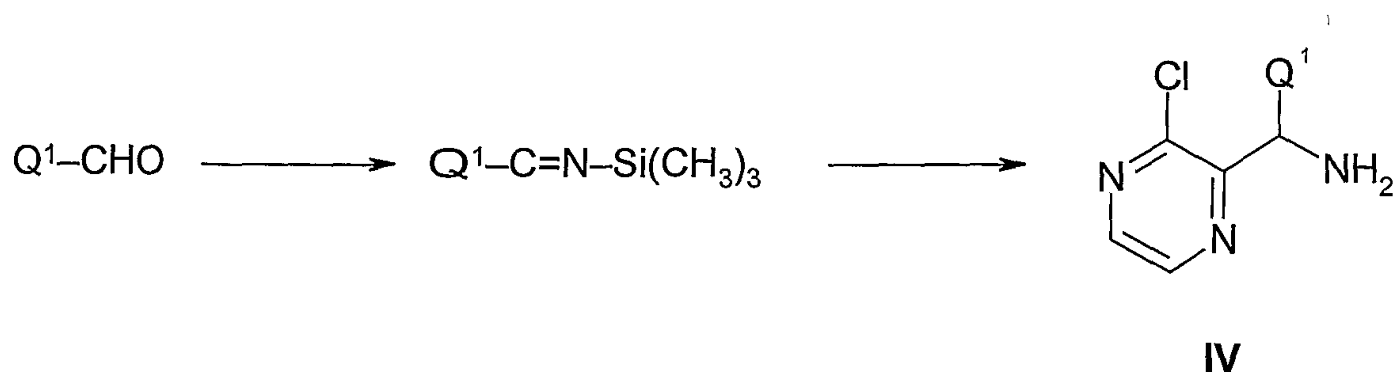
Scheme 4a
