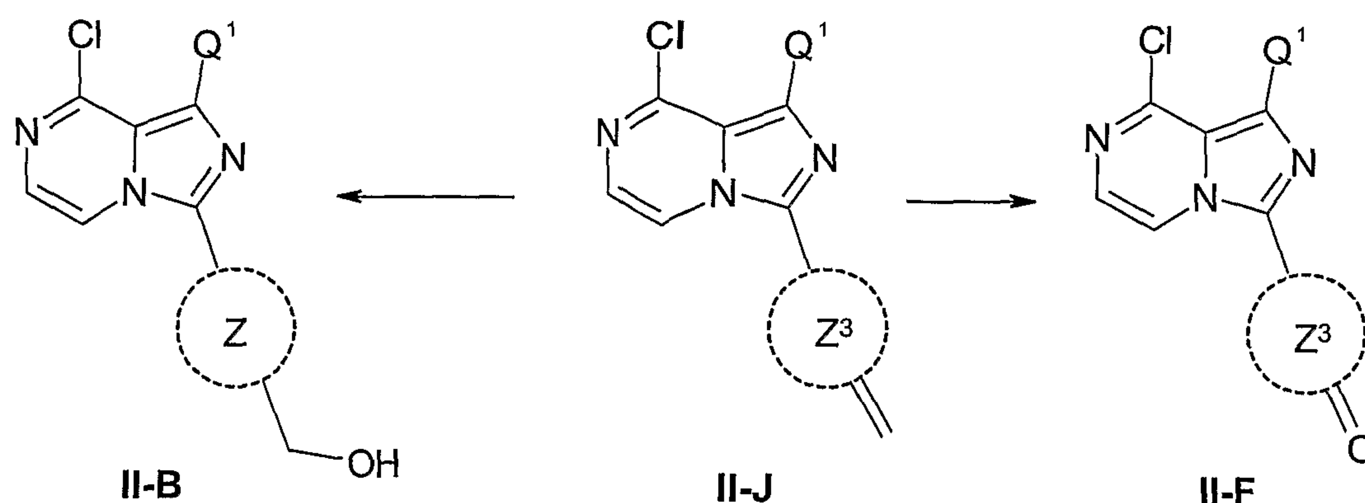
Scheme 11
