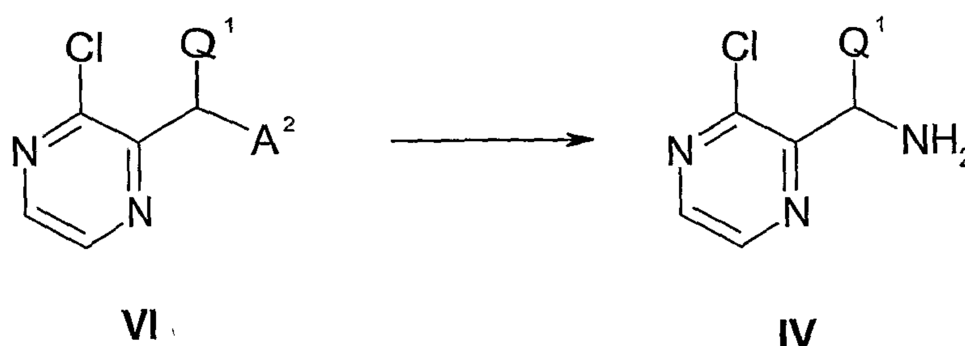
Scheme 4
