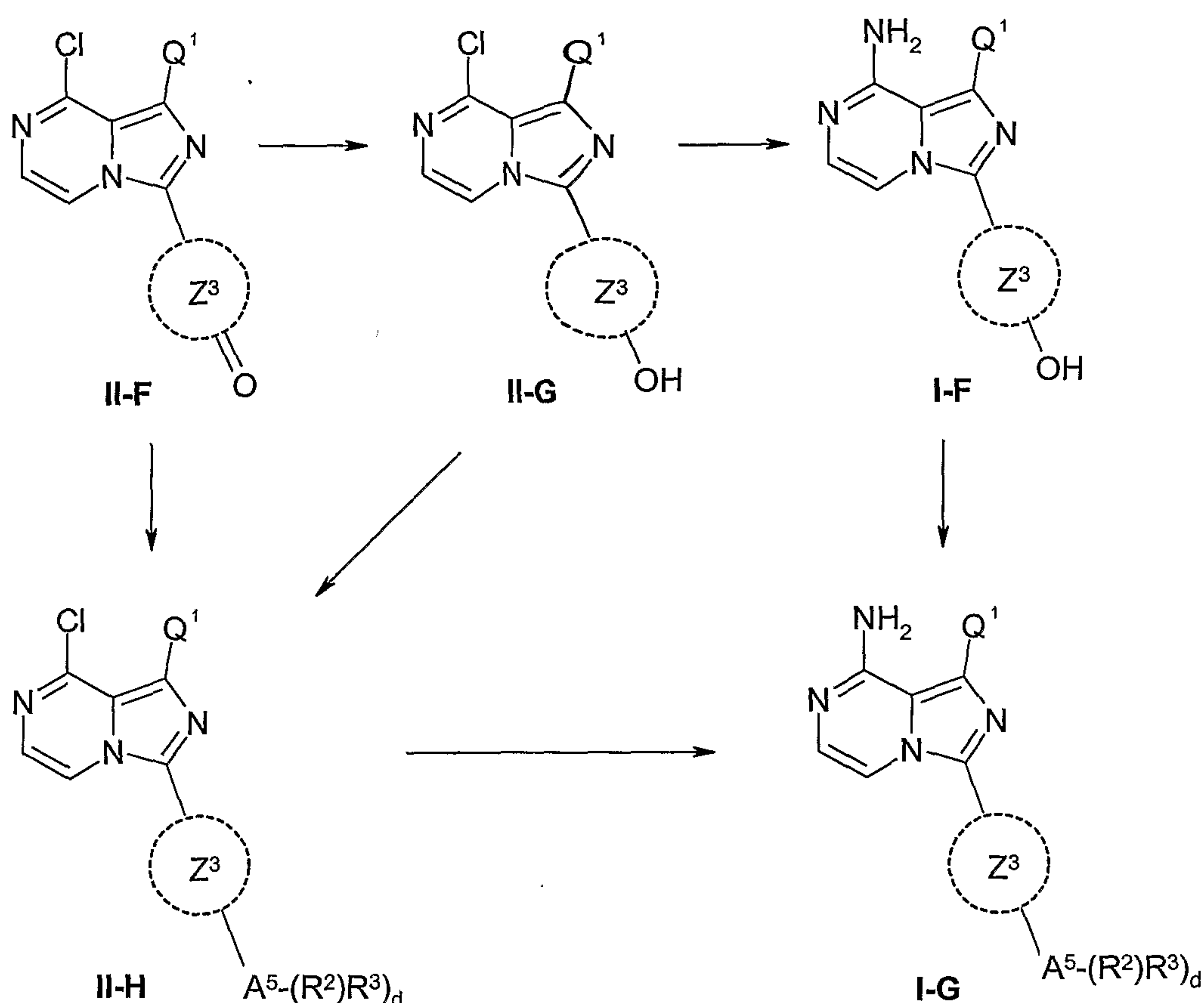
Scheme 10
