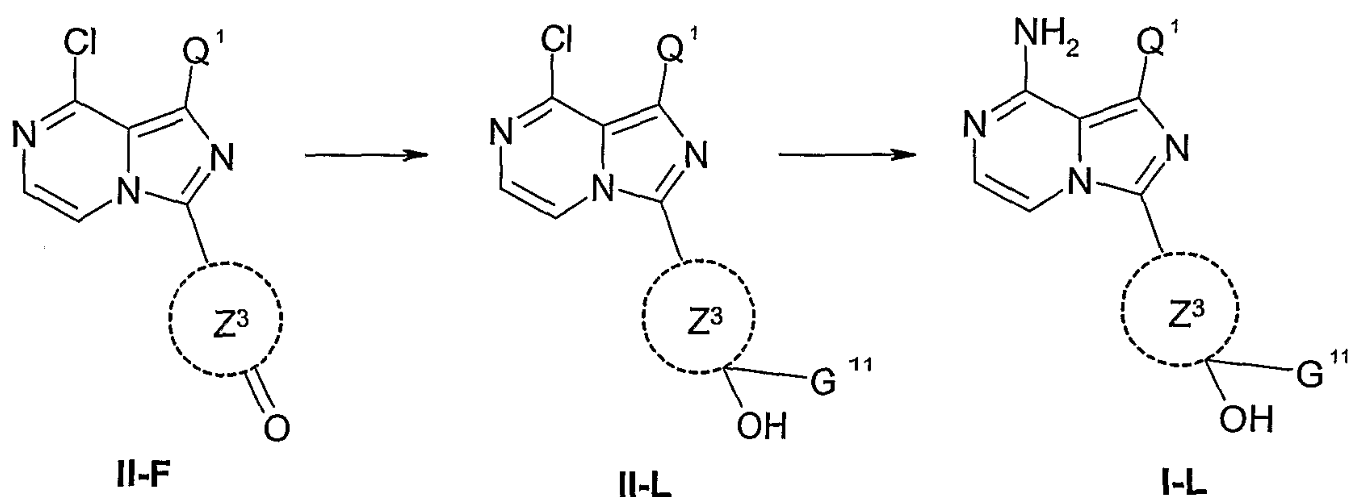
Scheme 13
