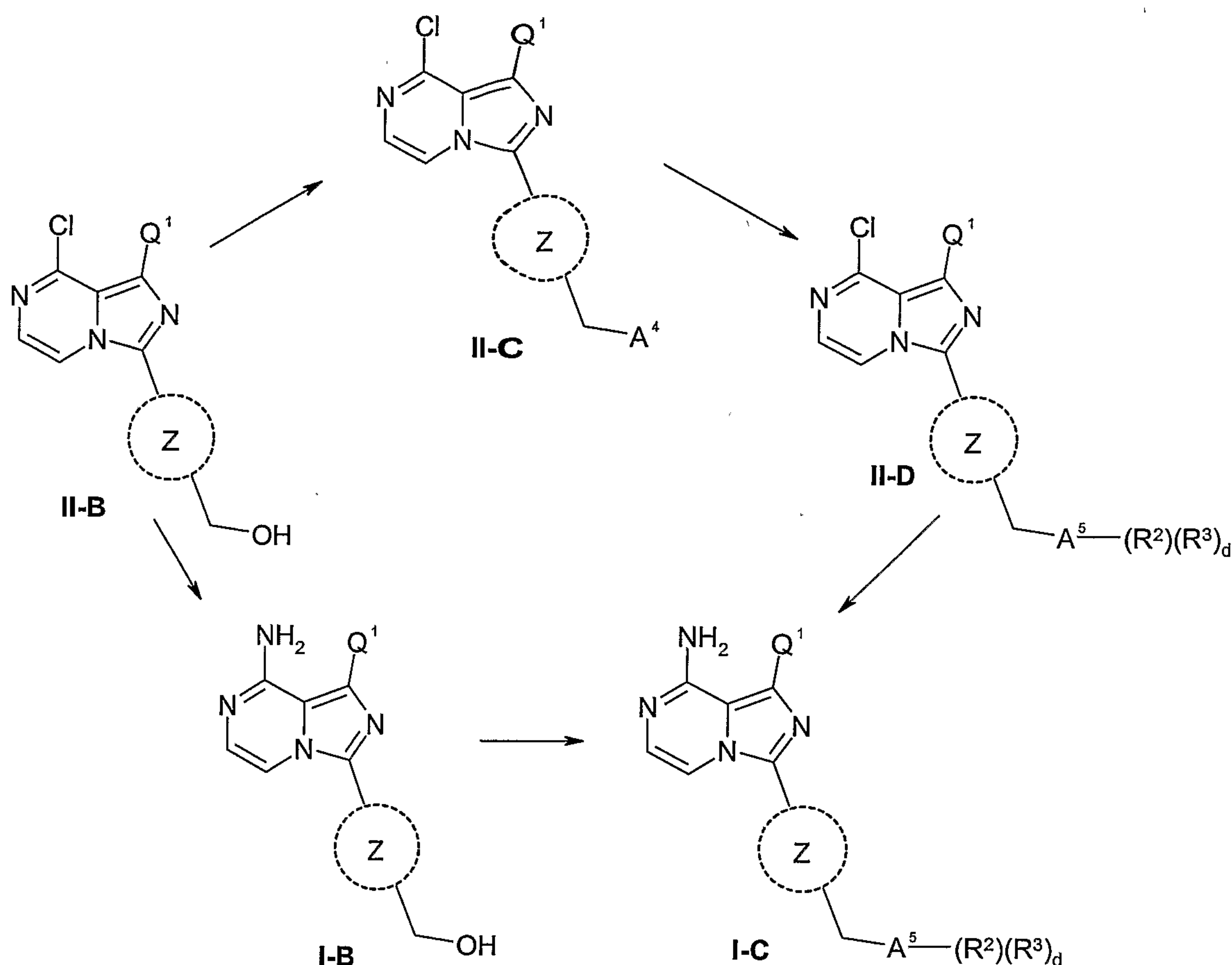
Scheme 8
