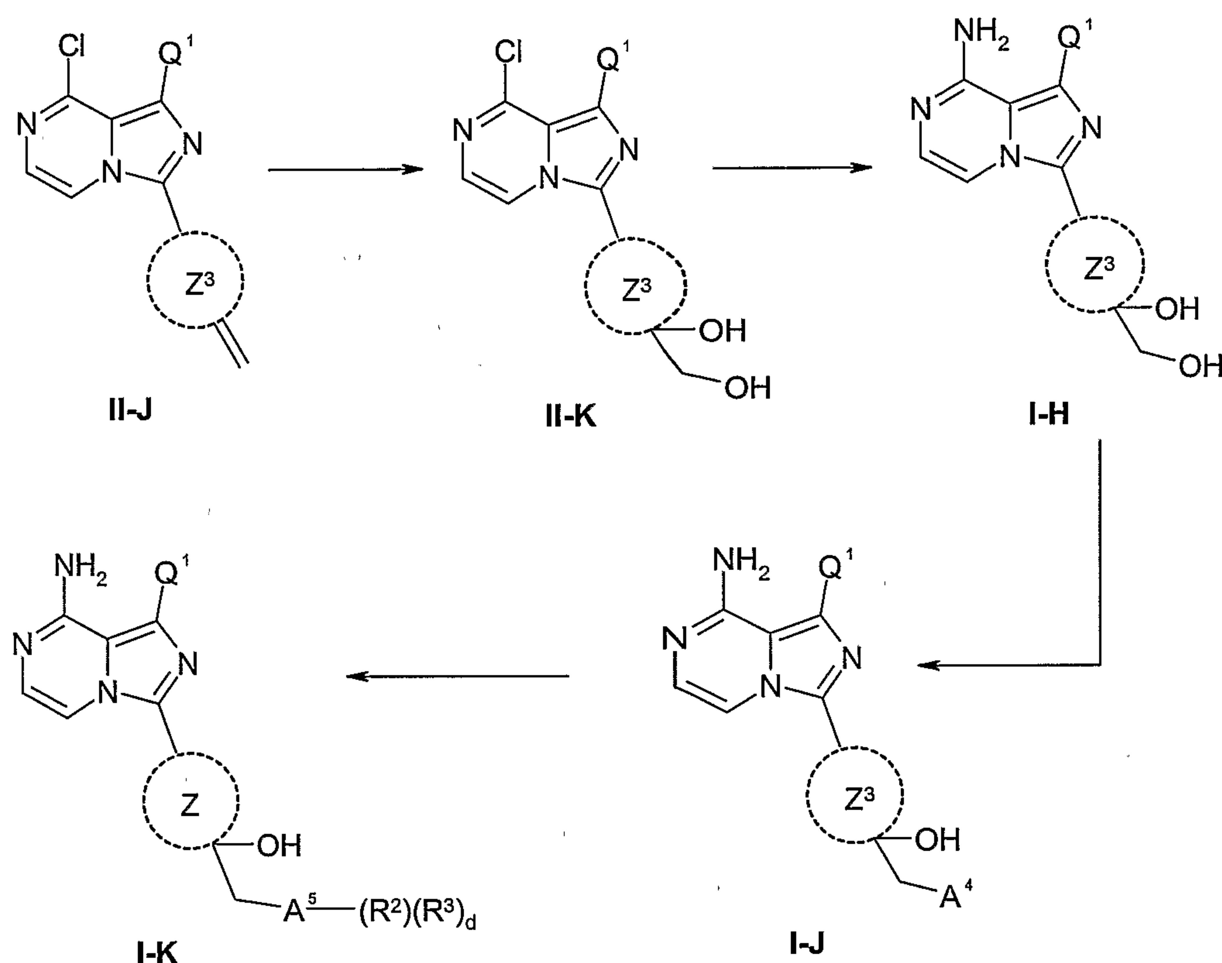
Scheme 12
