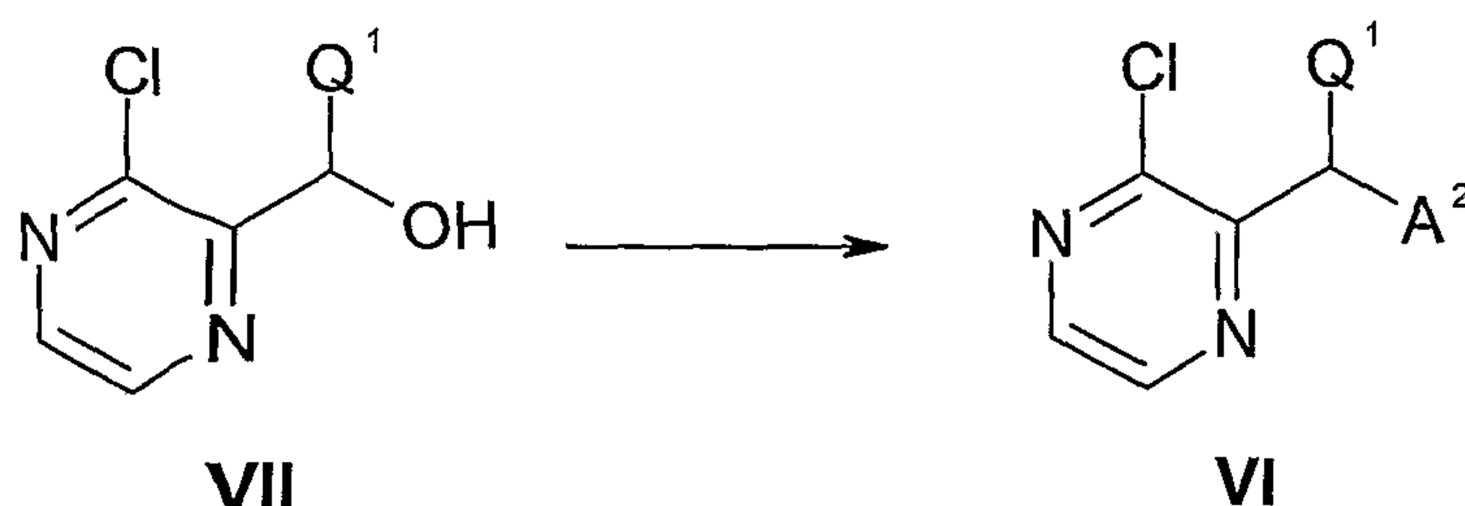
Scheme 5
