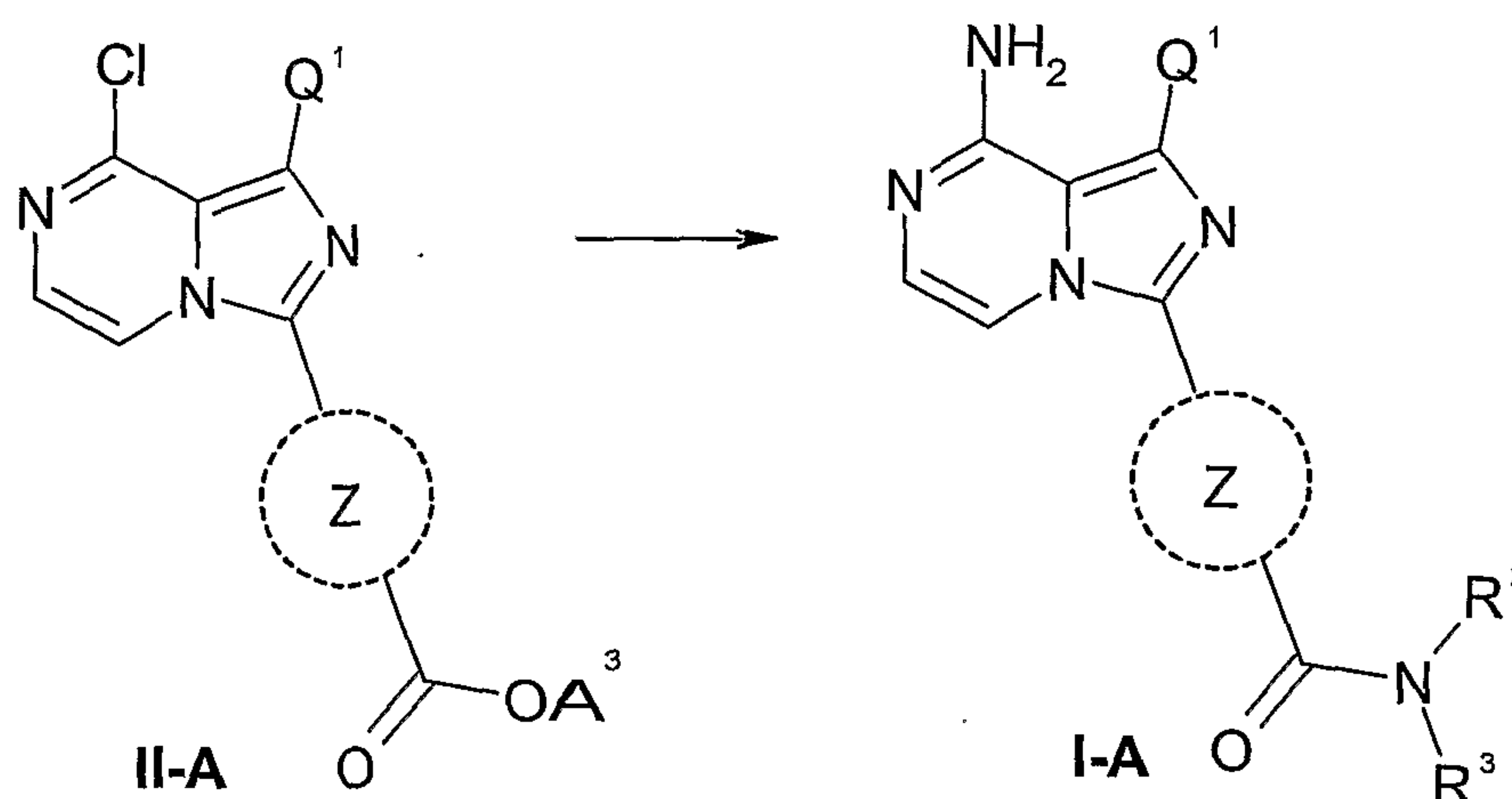
Scheme 6
