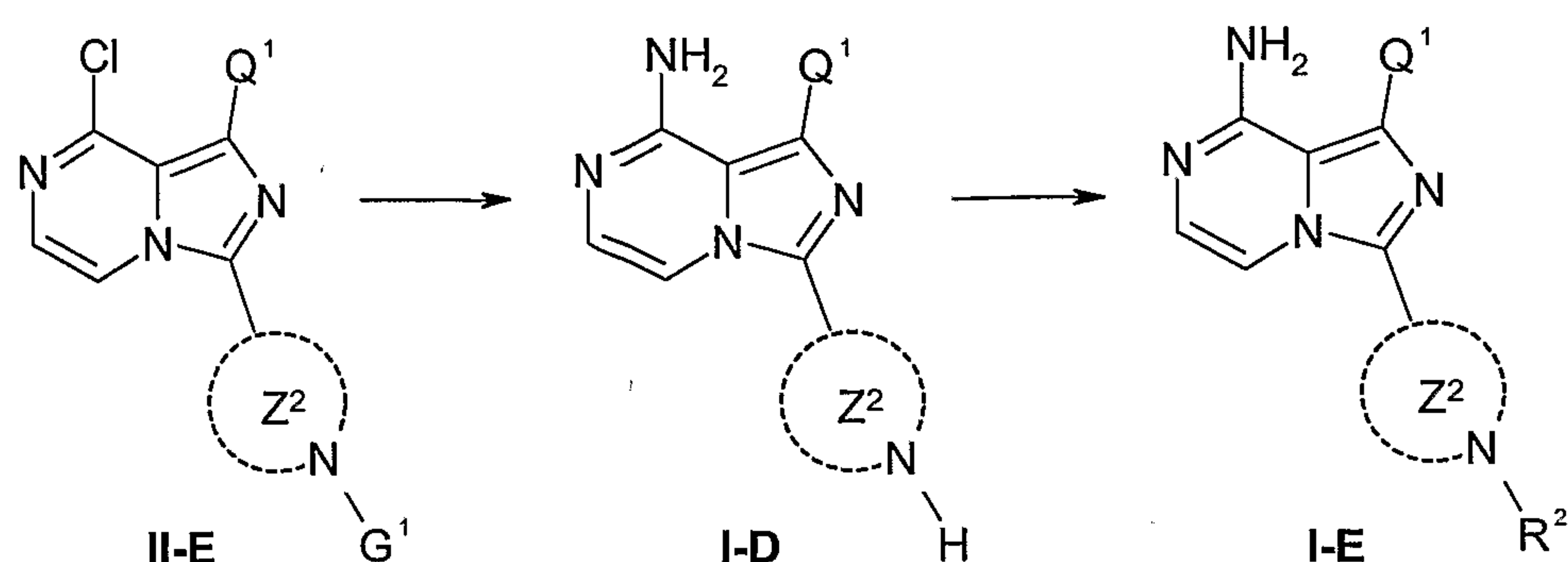
Scheme 9
