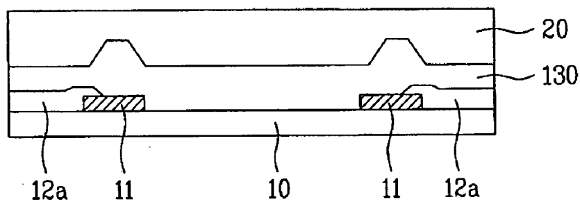
FIG. 2C Related Art
