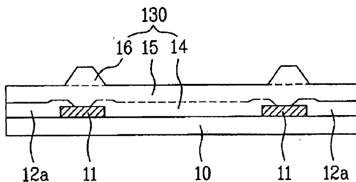
FIG. 2C Related Art
