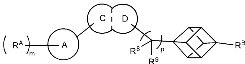
Formula (VI)
