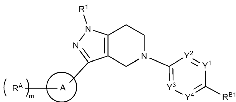
Formula (IVa-2).
