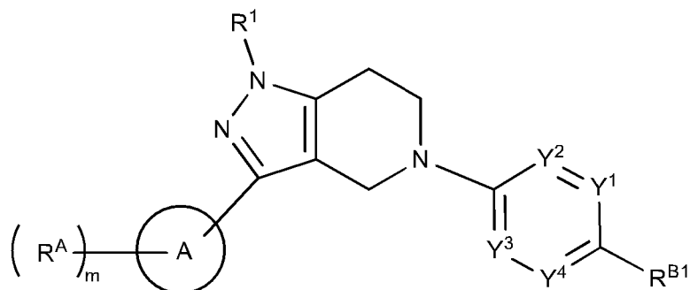
Formula (IVa-2).
