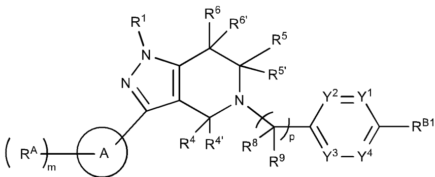
Formula (IVa)
