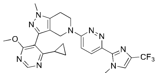
Compound 29
