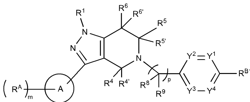
Formula (IVa),
