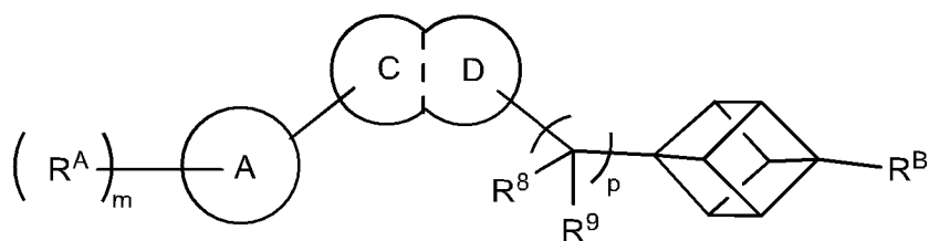
Formula (VI)
