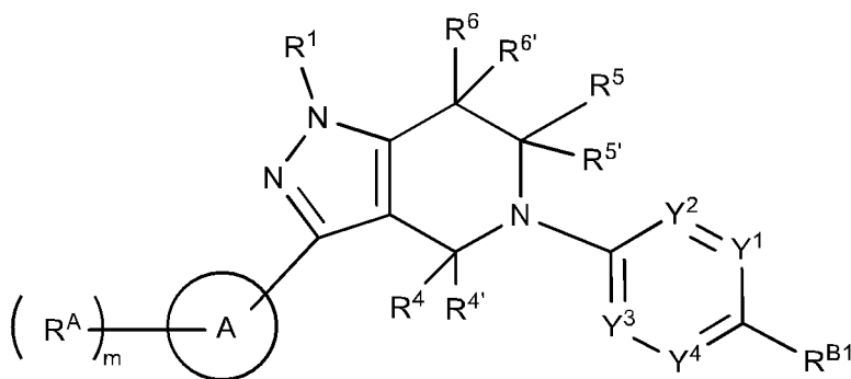
Formula (IVa-1).
