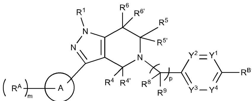
Formula (IVa)
