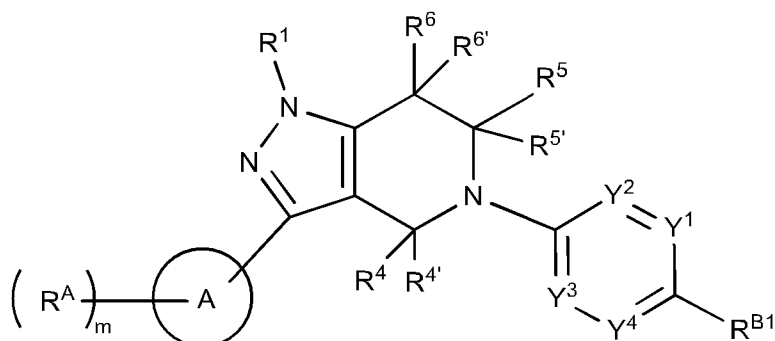
Formula (IVa-1).
