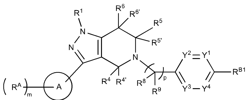
Formula (IVa)
