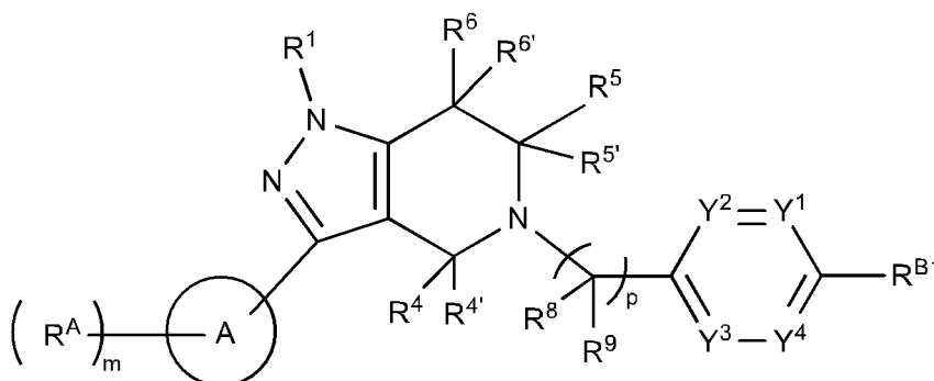
Formula (IVa)
