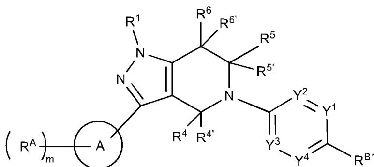
Formula (IVa-1).
