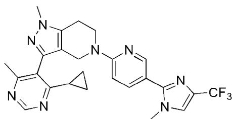
Compound 13
