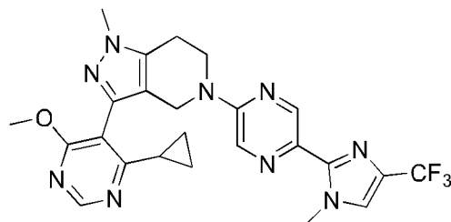
Compound 28
