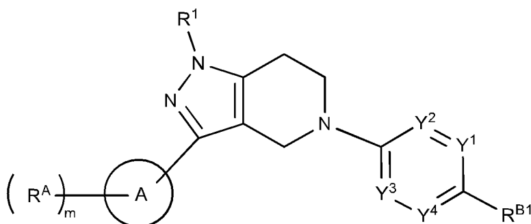
Formula (IVa-2).
