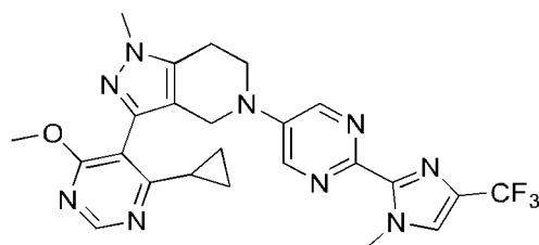
Compound 26
