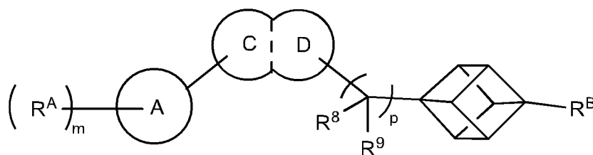
Formula (VI)
