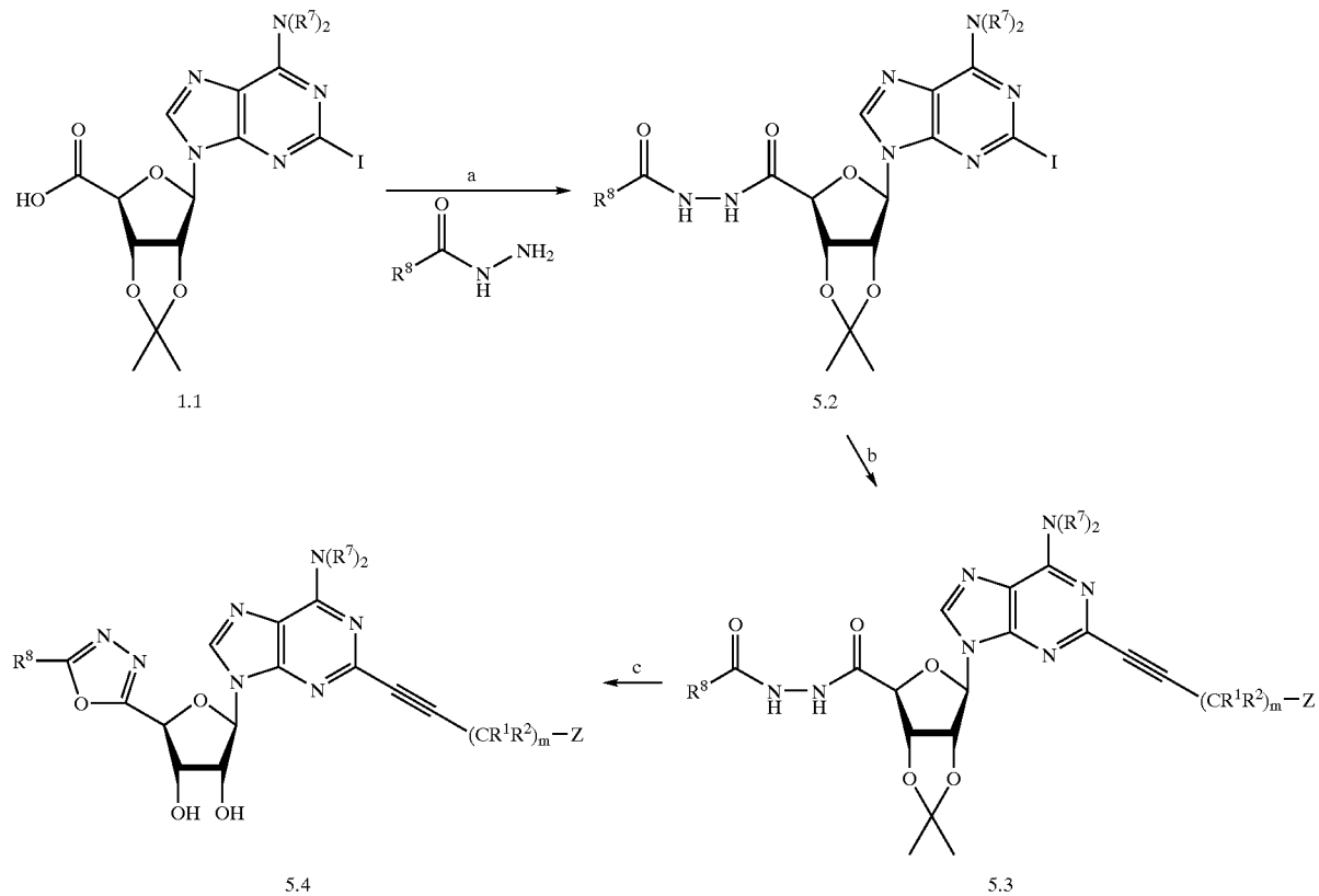
Scheme 5: Preparation of 4'-1,3,4-oxadiazoles
