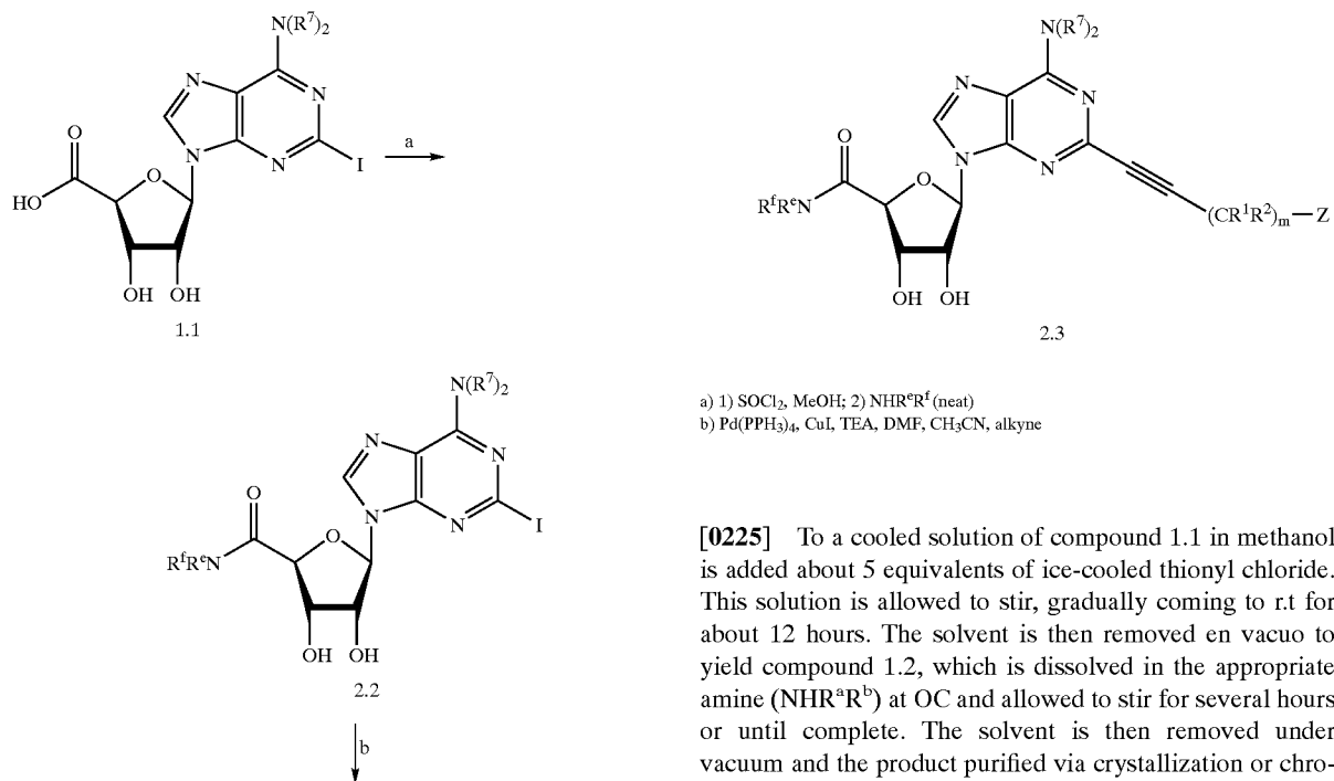
Scheme 2: Preparation of 5' amide analogs:
