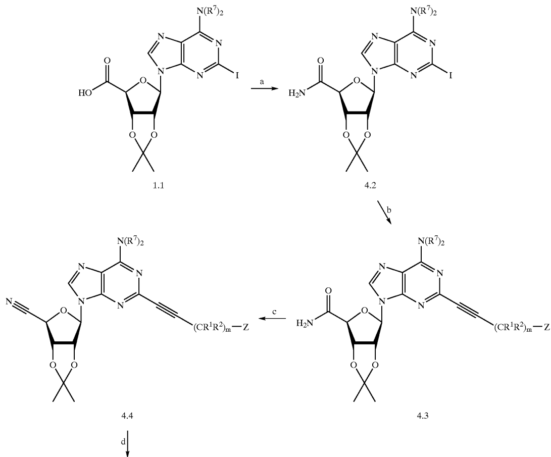
Scheme 4: Preparation of 4'-1,2,4-oxadiazoles
