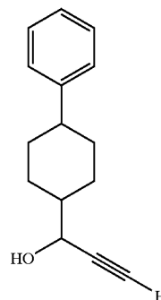
1-Ethynyl-4-phenyl-cyclohexanol (JR3153)
