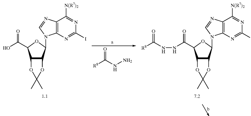
Scheme 7: Preparation of 4'-1,3,4 thiaziazole
