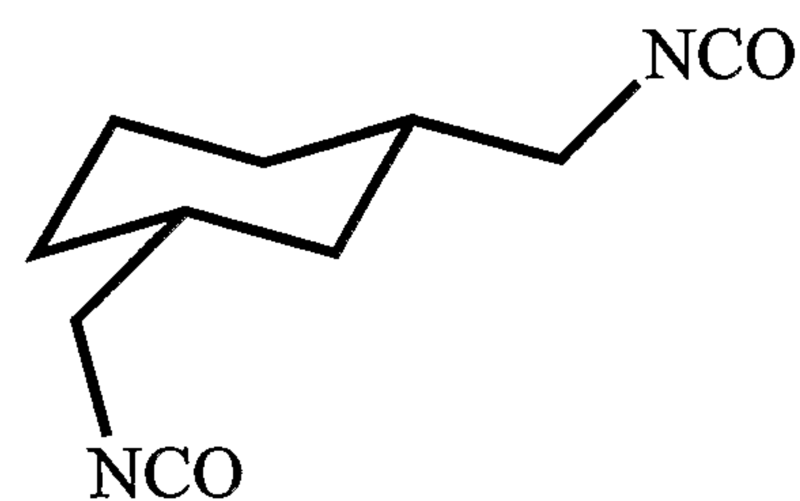
cis-1,3-bis(isocyanatomethyl)- cyclohexane Formula II
