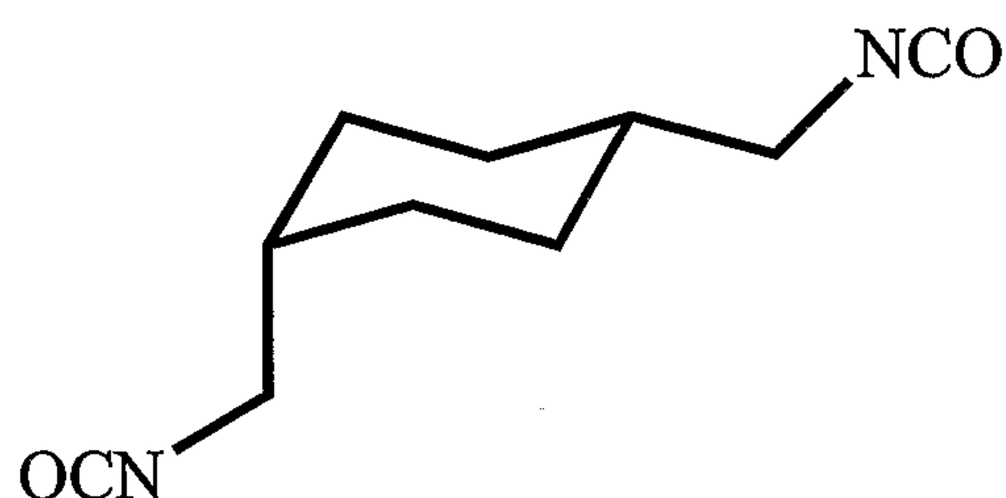
cis-1,3-bis(isocyanatomethyl)- cyclohexane Formula II
