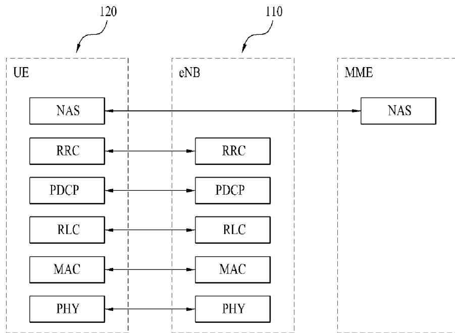
(a) Control-plane protocol stack
