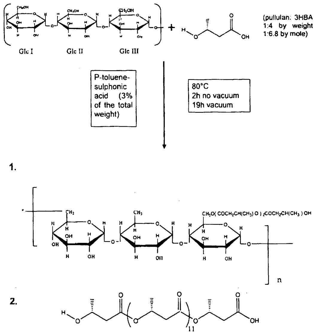
1. Modified pullulan and 2. PHB oligomers
