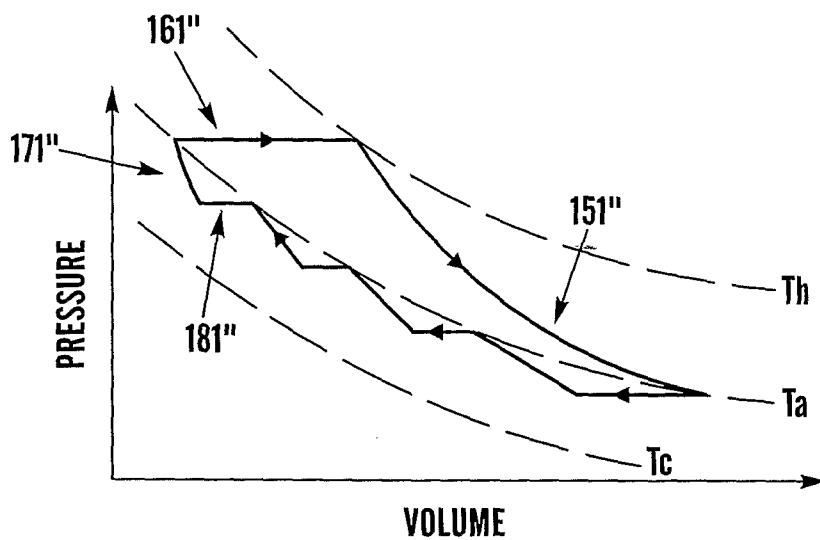
DISCHARGING ENERGY - COLD SYSTEM (HYBRID)
