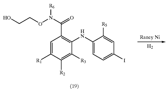
Scheme 10 Representative Hydrogenolysis of Aryl Iodides
