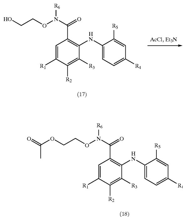
Scheme 9 Representative Preparation of Acetates by Acetylation
