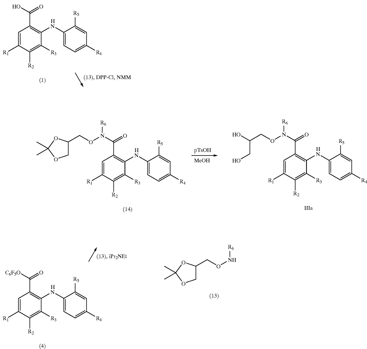
Scheme 7 Representative Preparation of Dihydroxylated Benzamides Using an Acetonide as a Diol Protecting Group
