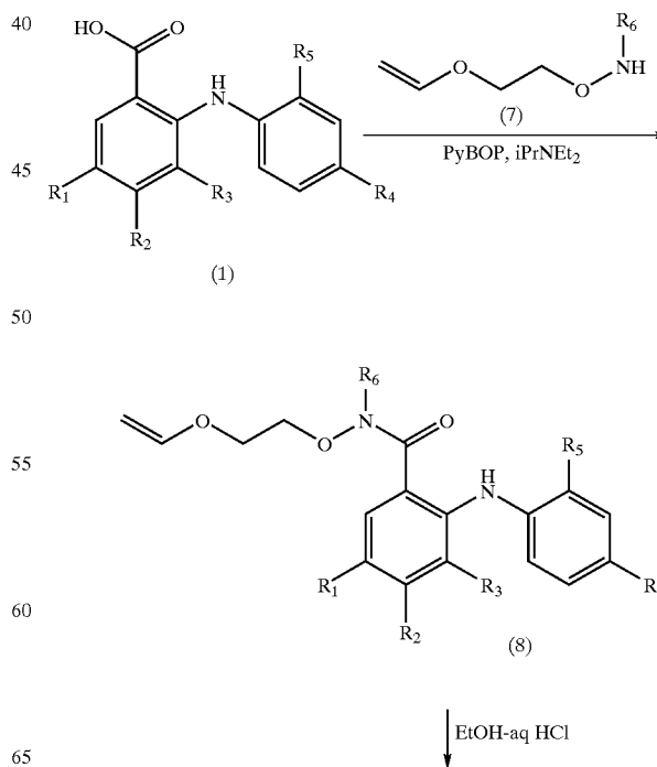
Scheme 4 Representative Preparation of Hydroxylated Benzamides Using a Vinyl Ether as a Hydroxyl Protecting Group
