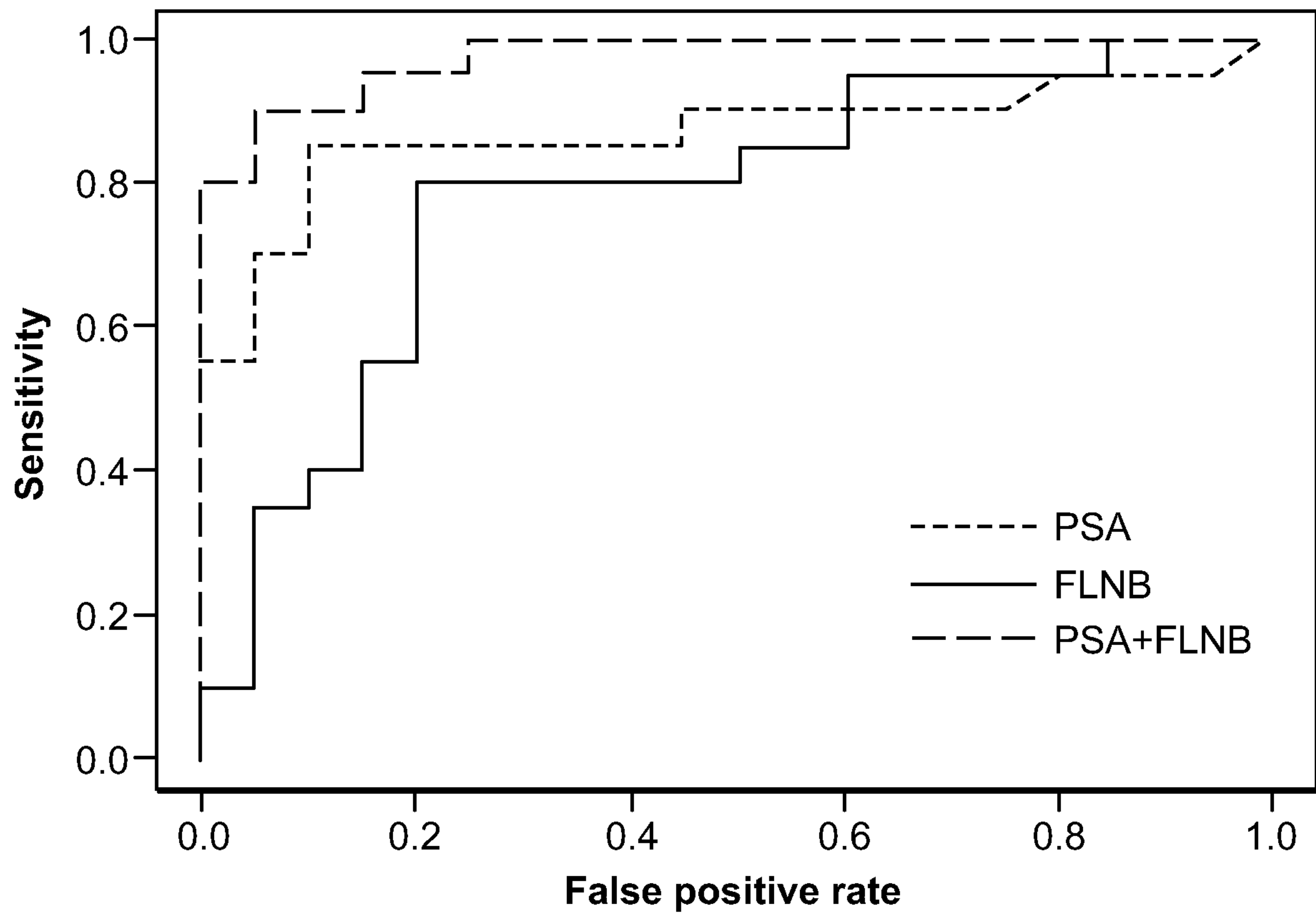
ROC curves for PSA, FLNB and combination
