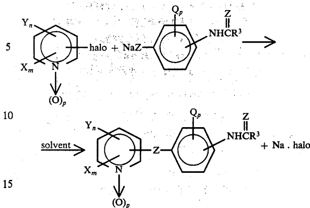
Reaction I
