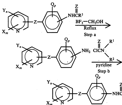
Reaction II
