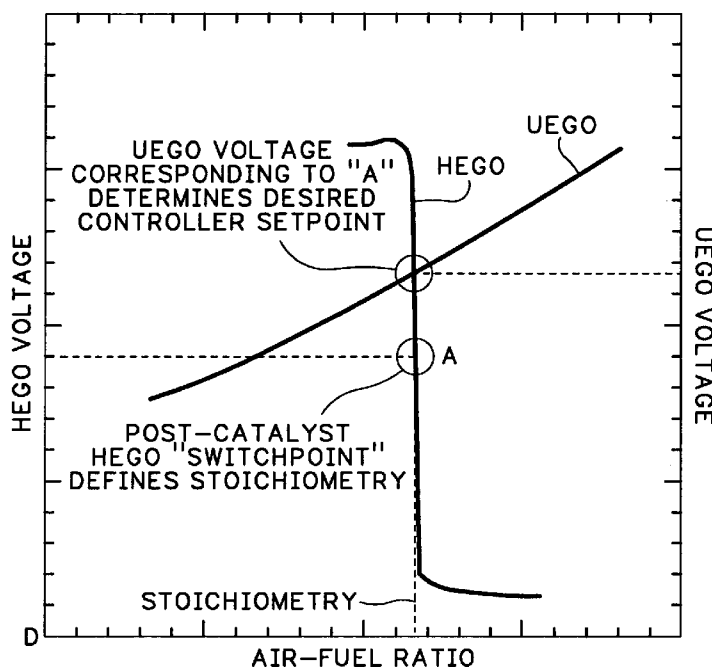
COMBINED UHEGO-HEGO SENSOR OUTPUT VOLTAGES
