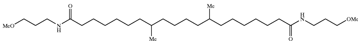
Amphipathic amide lipid A
