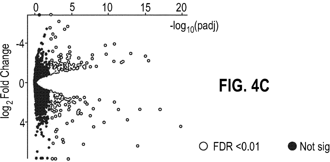
Comparison of active and quiescent Lgr5 signatures
