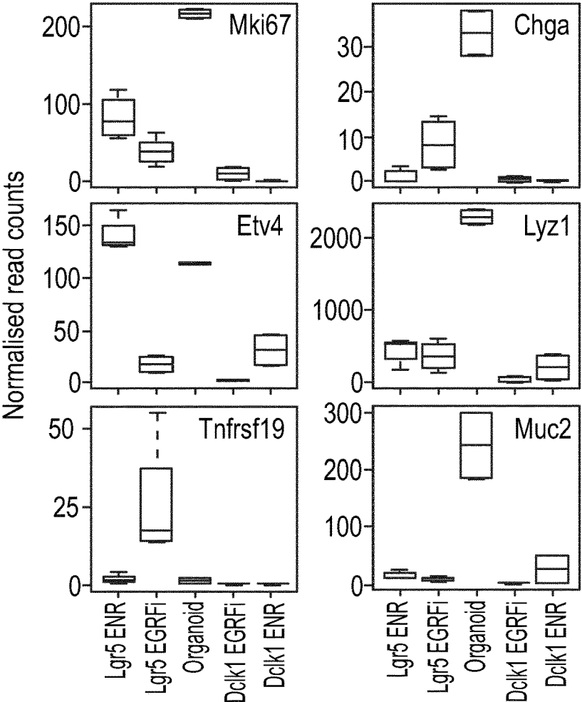
Marker gene expression
