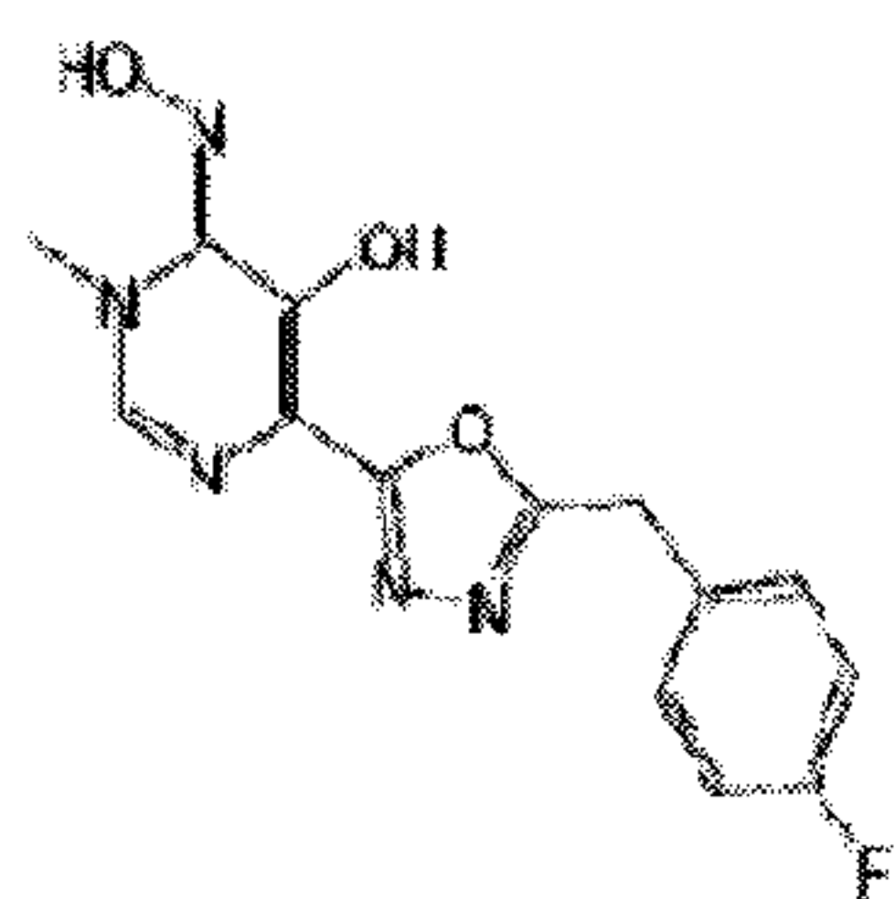
COTI-HIV-1 Formula: C_{14}H_{12}FN_5O_3 Mol. weight: 317.09 g/mol
