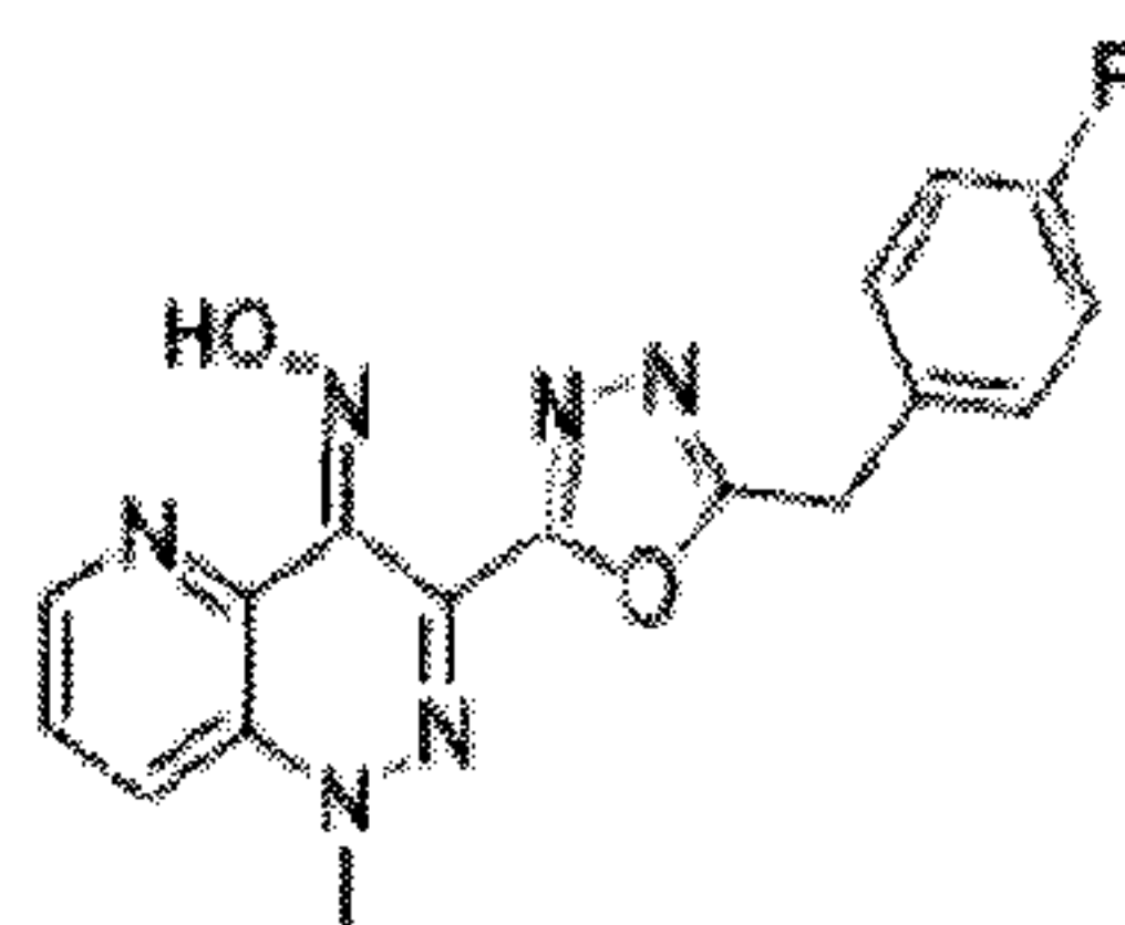
COTI-HIV28233 Formula: C_{17}H_{13}FN_6O_2 Mol. weight: 352.32 g/mol
