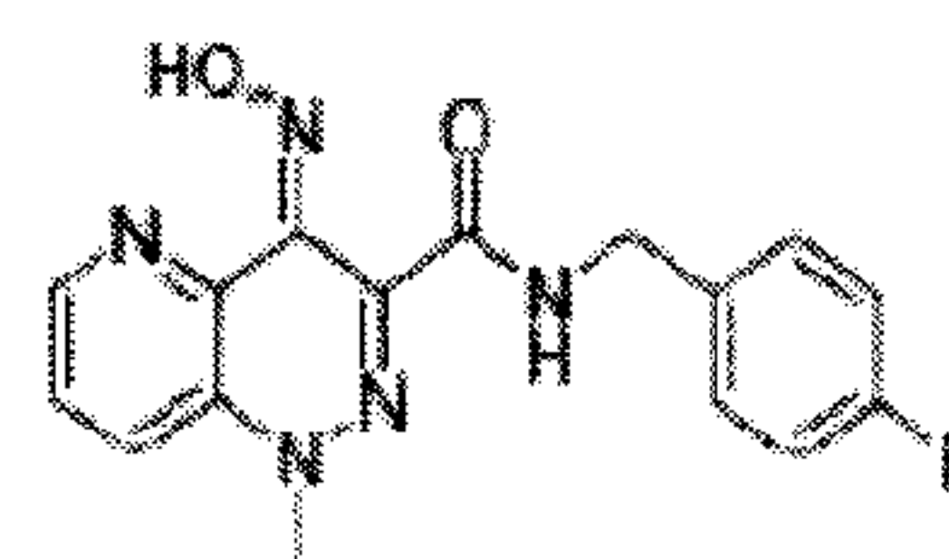
COTI-HIV28236 Formula: C_{16}H_{14}FN_5O_2 Mol. weight: 327.31 g/mol
