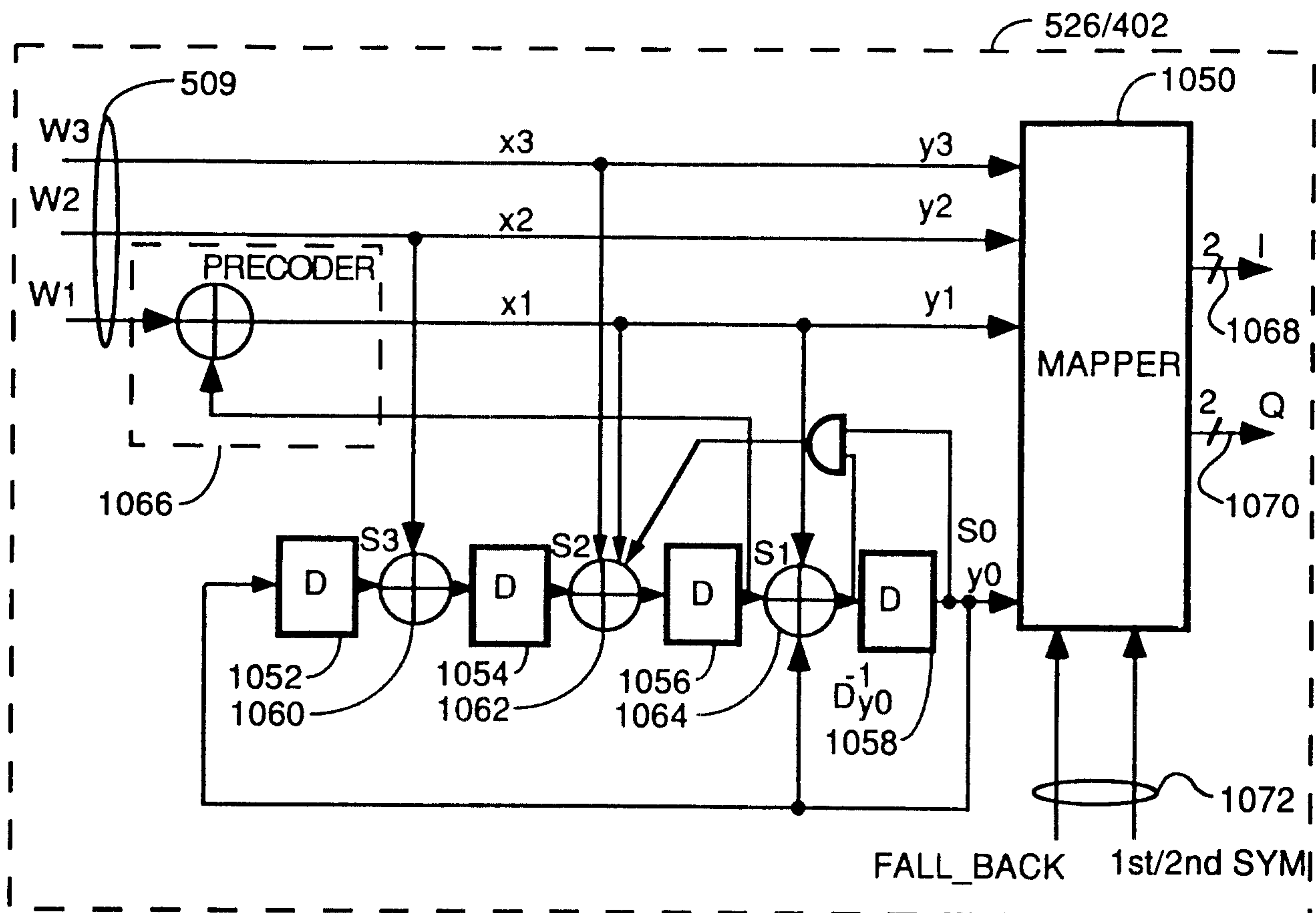
PREFERRED TRELLIS ENCODER
