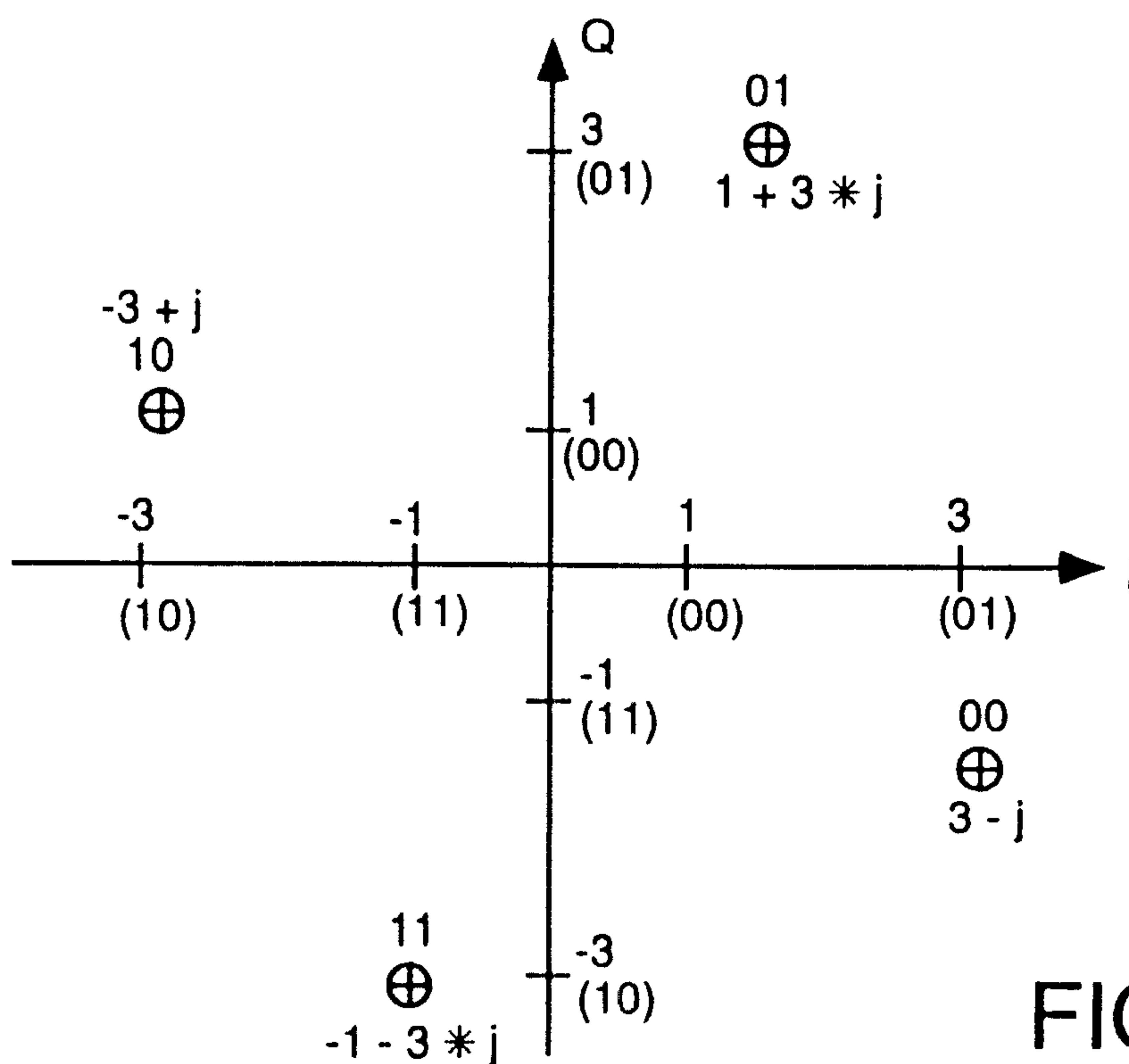
MAPPING FOR FALL-BACK MODE - LSB'S
