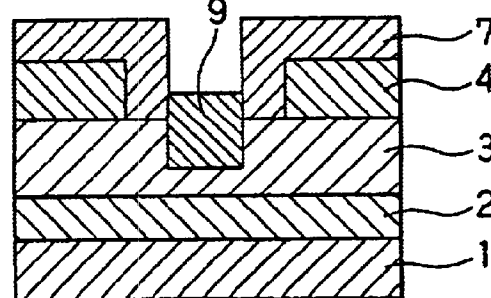
FIG. 1C (Prior Art)
