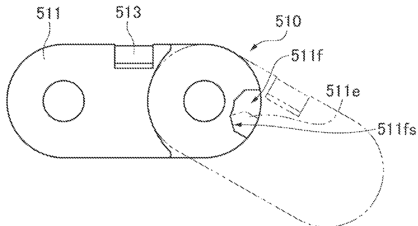
FIG. 14 PRIOR ART
