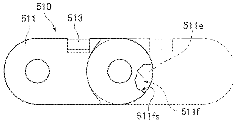
FIG. 13 PRIOR ART
