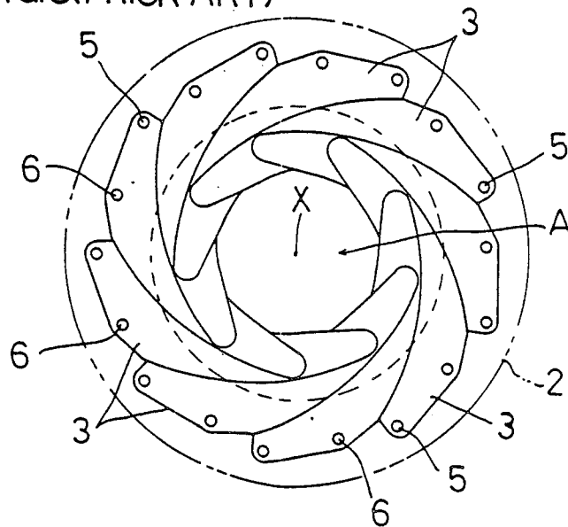
FIG. 8 (PRIOR ART)
