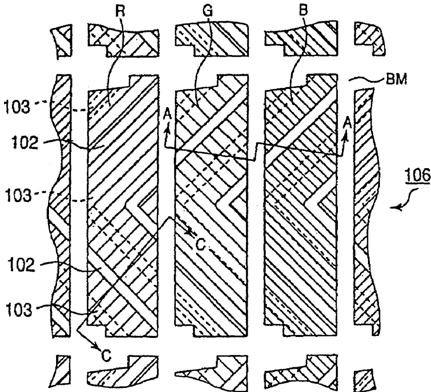
PRIOR ART FIG.35
