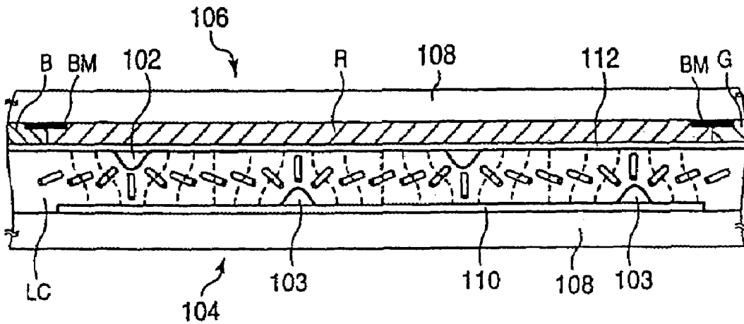
PRIOR ART FIG.38
