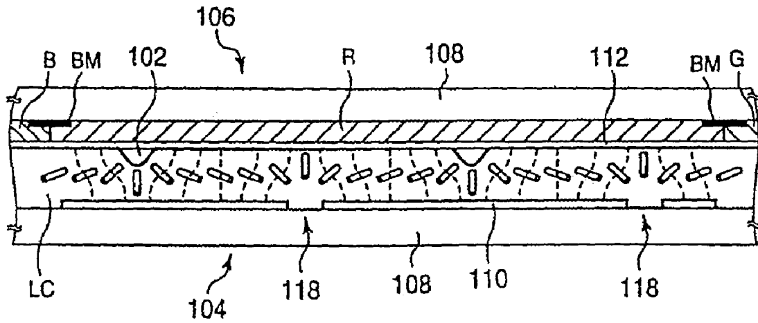
PRIOR ART FIG.39
