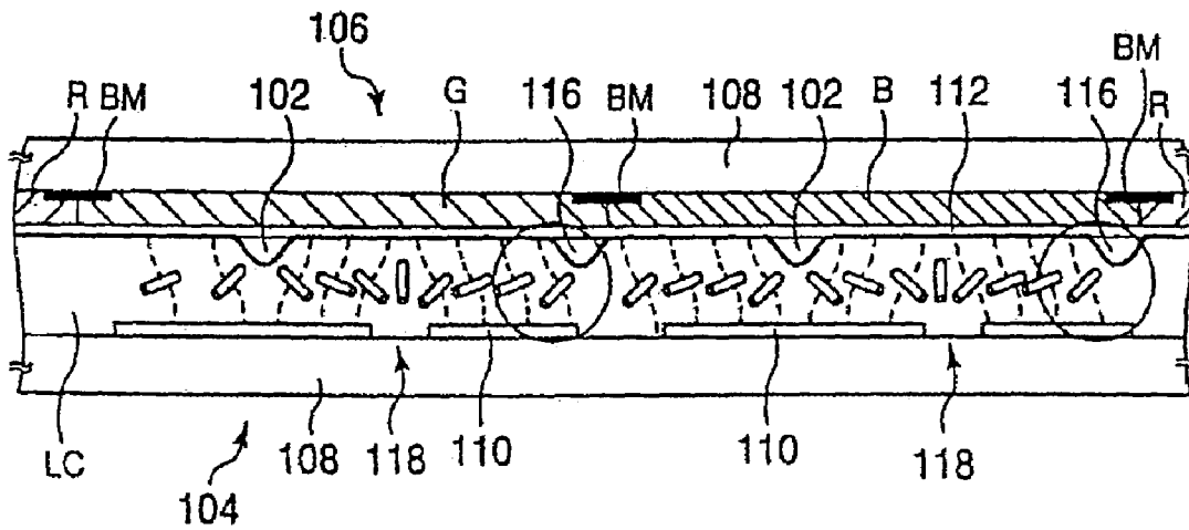
PRIOR ART FIG.42
