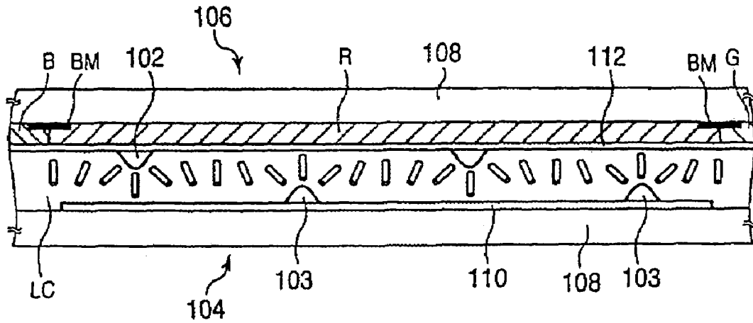
PRIOR ART FIG.37
