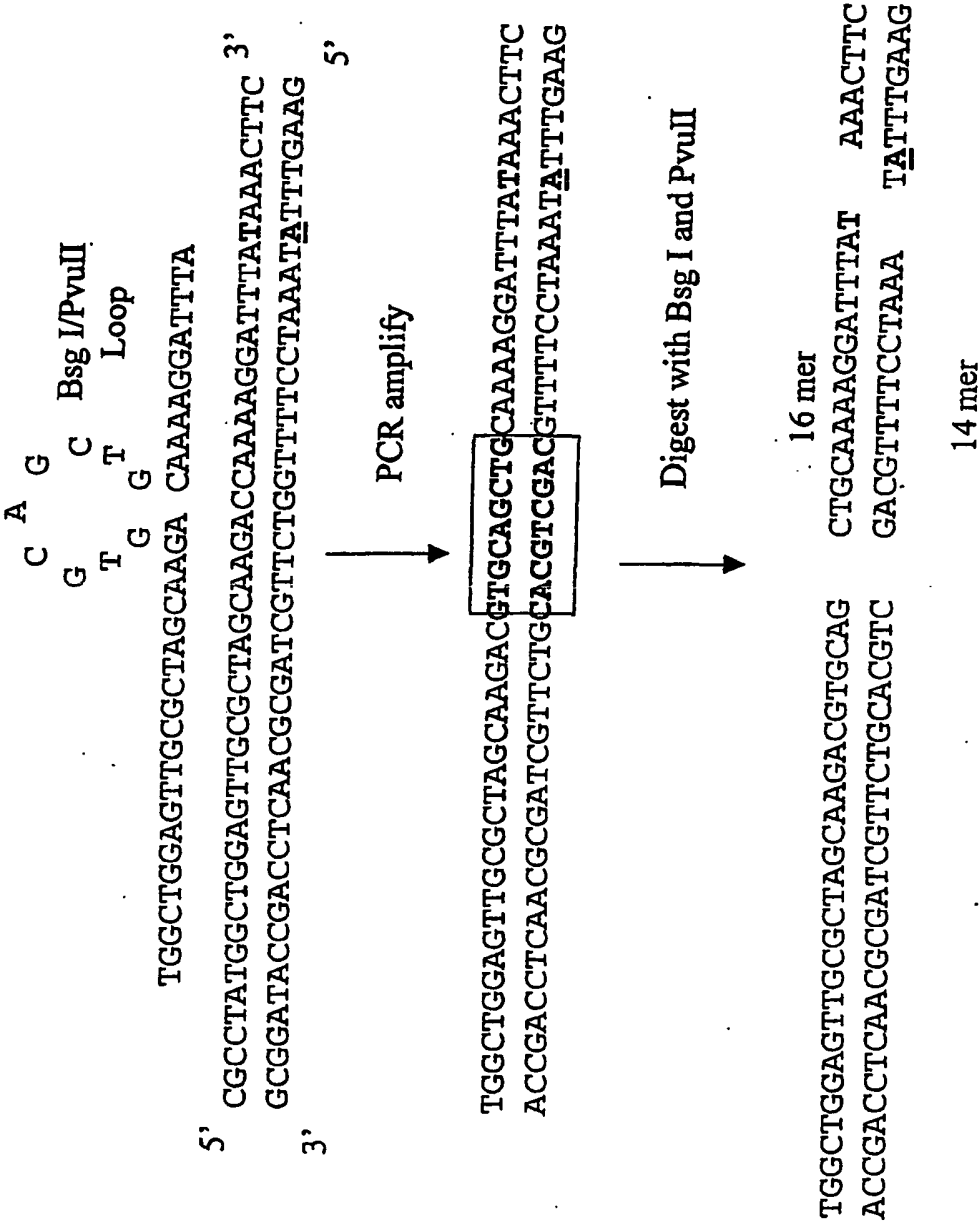
Introduction of Bsg I and Pvu II sites during PCR by loop followed by endonuclease digestion.
