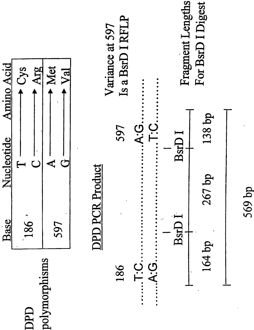
FIG. 21 Dihydropyrimidine dehydrogenase (DPD) polymorphisms used in haplotyping assay.
