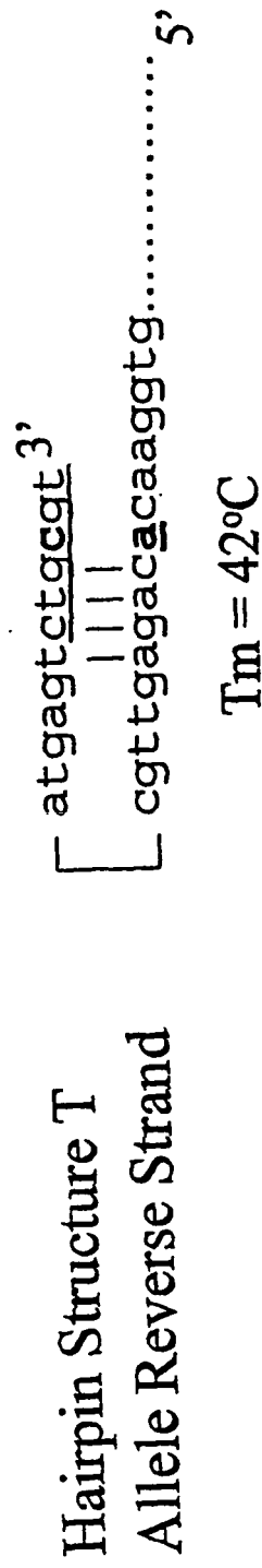
FIG. 28 Hairpin Structures for PCR Products Generated Using DPDASTF Primer
