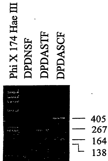
BsrD I Digest of Allele Specific PCR Products.
