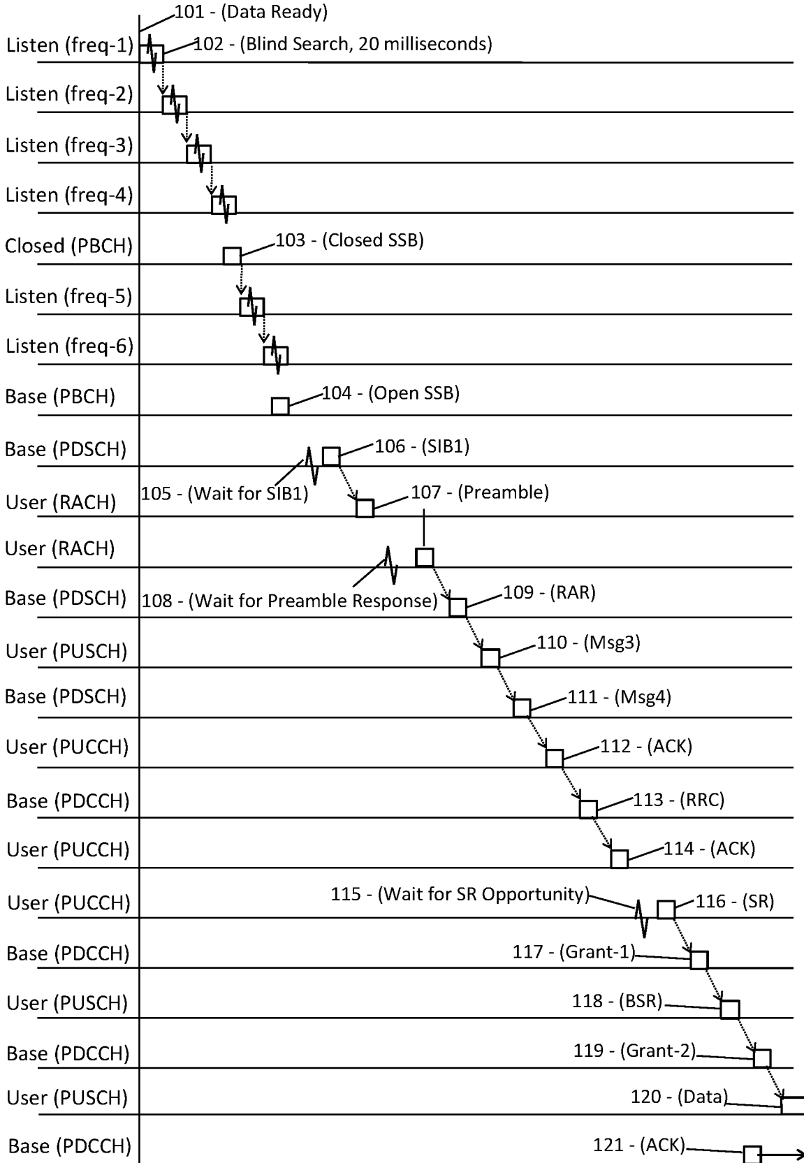
FIG. 1 (prior art)
