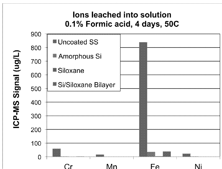
FIG. 3. Comparison of ions leached into solution from 2x3 cm stainless steel coupons coated with a-Si, siloxane, and Si/Siloxane bilayer compared to ions leached from uncoated stainless steel. Coupons were soaked in 0.1% formic acid at 50C for four days. Metal ion concentration in solution measured by Inductively Coupled Plasma-Mass Spectrometry.
