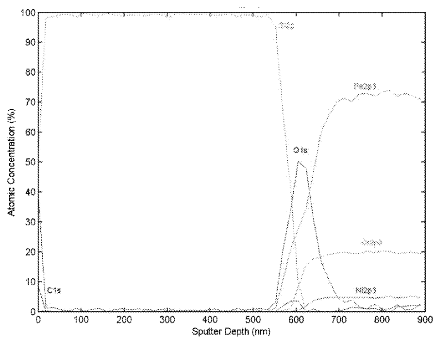
FIG. 2. X-ray Photoelectron Spectroscopy compositional depth profile of a-Si coating on stainless steel.
