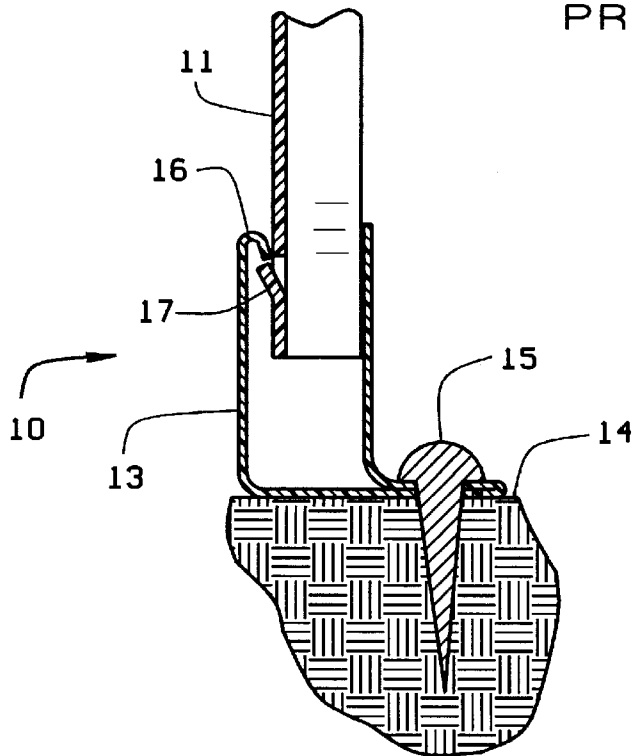
FIG. 2 PRIOR ART
