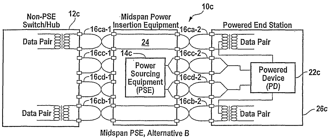
FIG. 1C (PRIOR ART)
