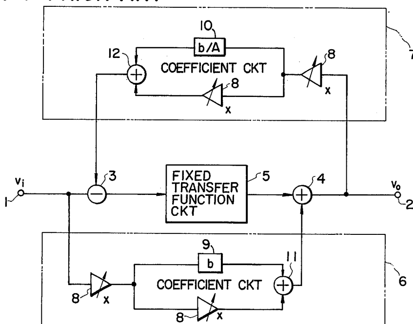
FIG. 4 PRIOR ART
