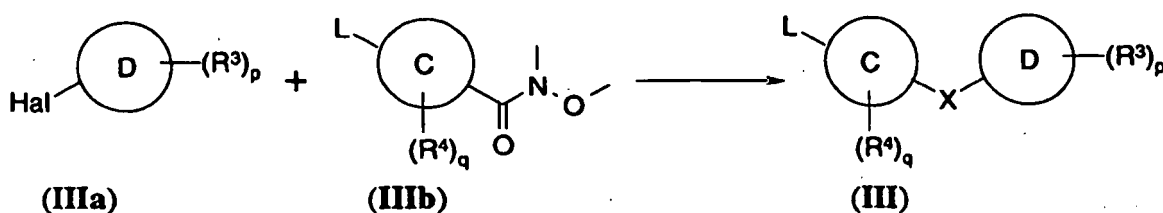
SCHEME V
