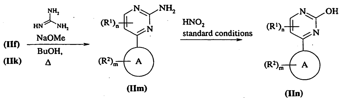
SCHEME IV
