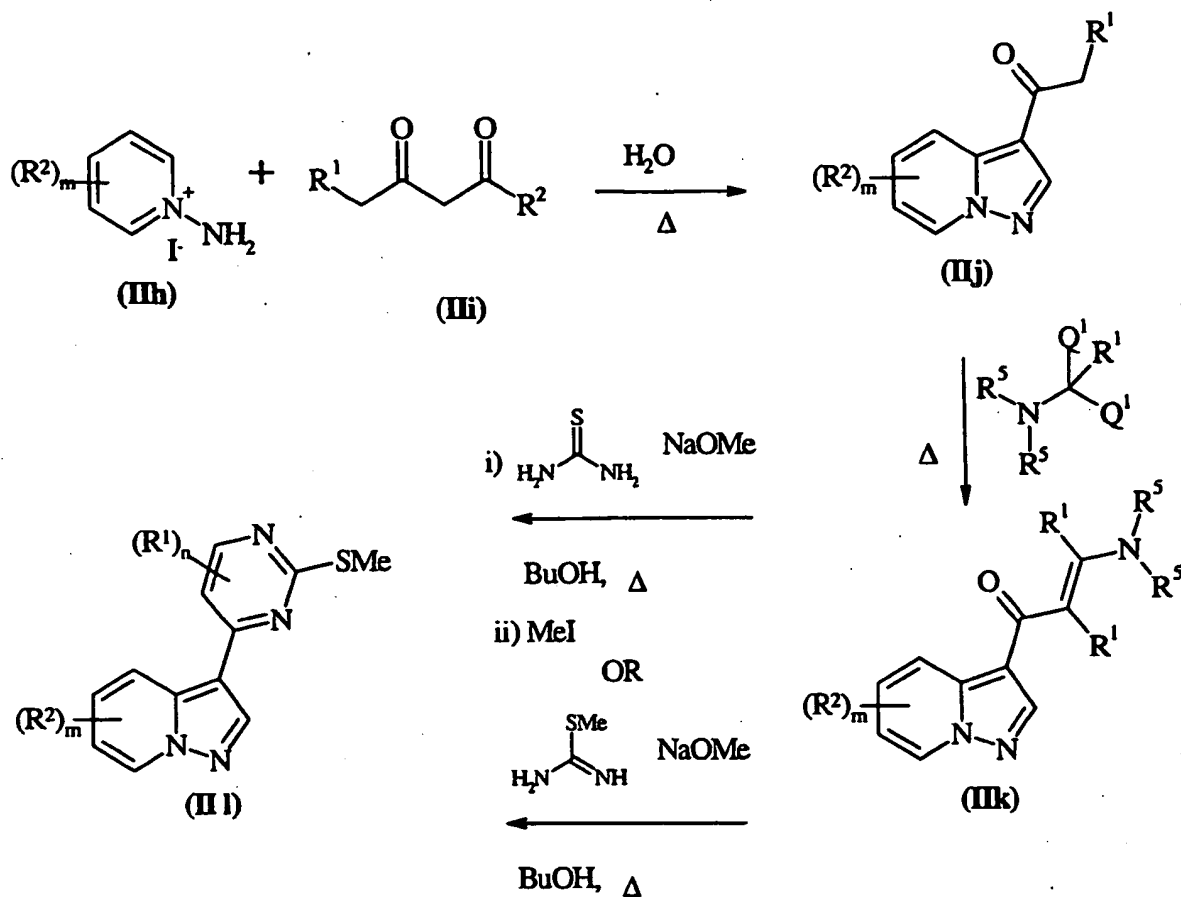
SCHEME III
