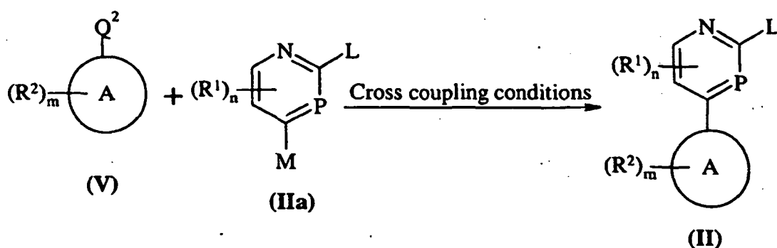
SCHEME I
