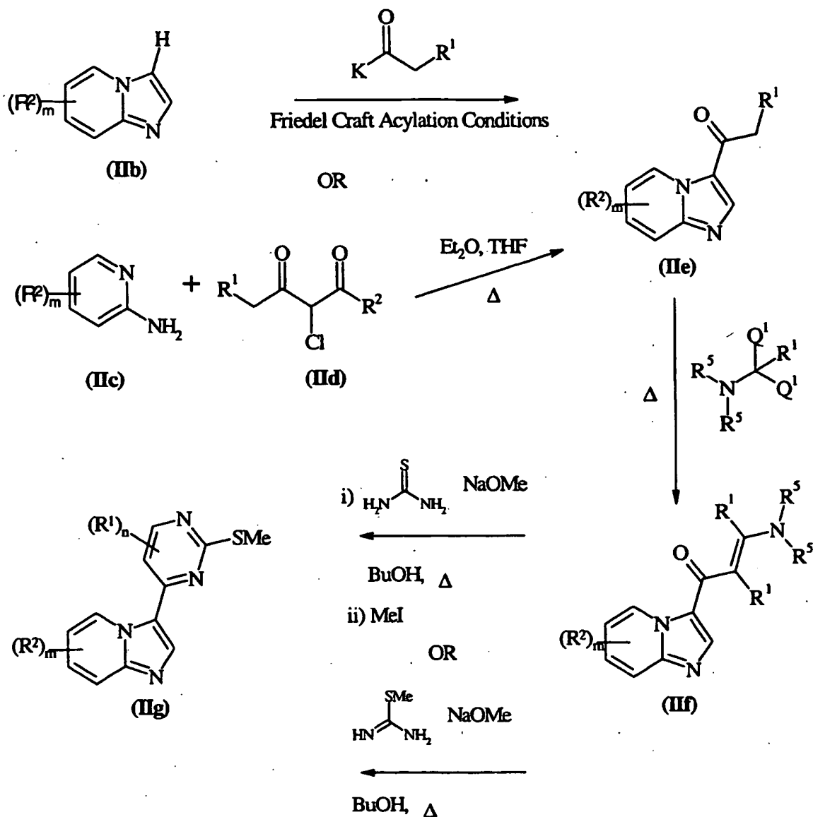
SCHEME II
