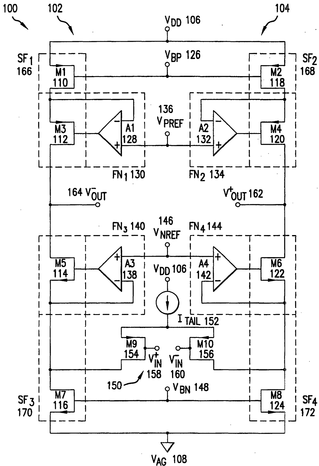
(CONVENTIONAL GAIN BOOSTED FOLDED CASCODE OPERATIONAL AMPLIFIER)
