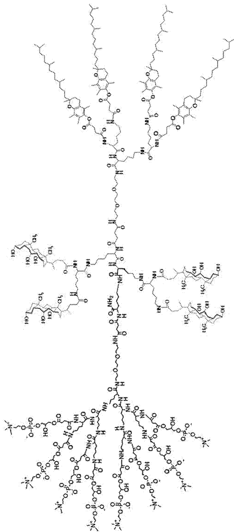
PC Janus dendrimer with segregated CA and CHO functionalities
