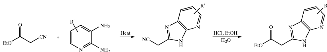
Scheme 5.
