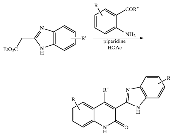
Scheme 4.
