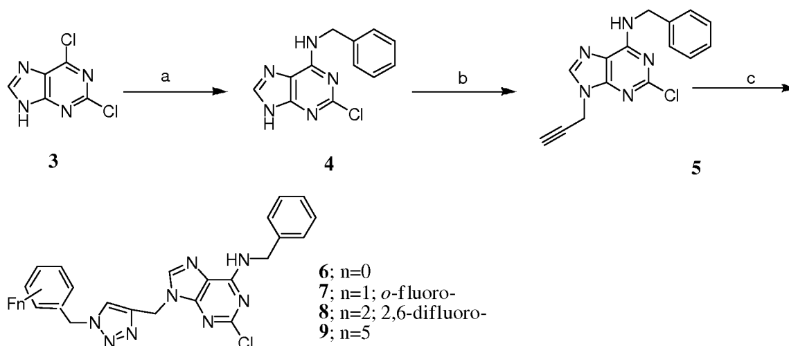
Scheme 1. Synthesis of purine-based fluoroaryl triazoles; reagents and conditions:
