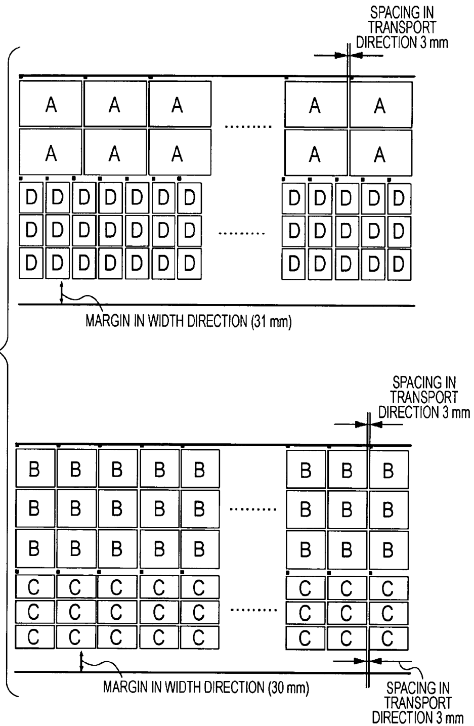
FIG. 10C THIRD PRINTING PROCESS
