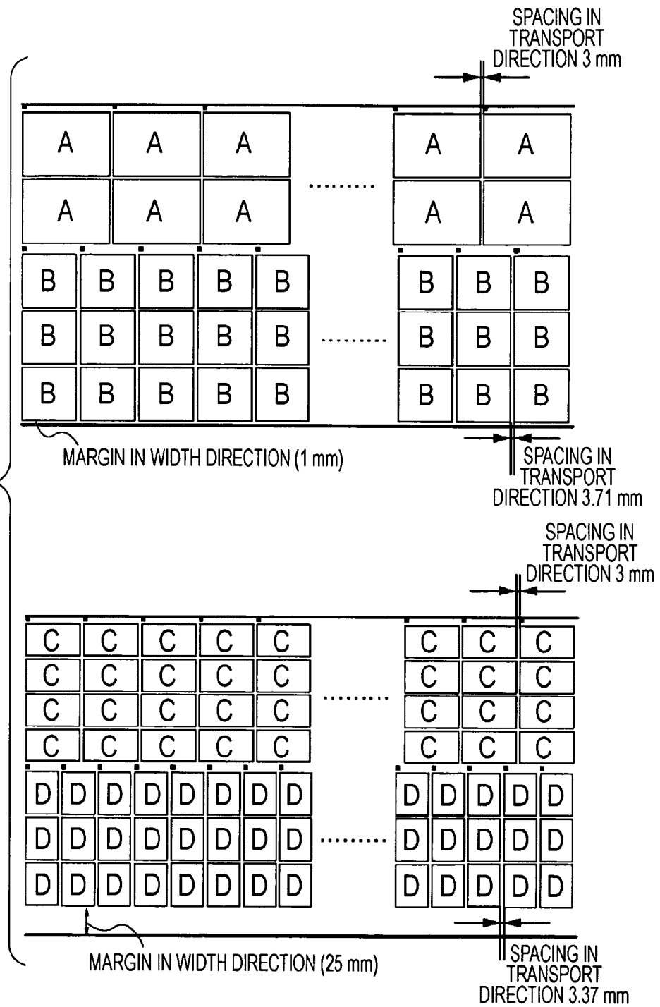
FIG. 10A FIRST PRINTING PROCESS
