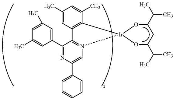
[Ir(dmprr-P) 2 (dibm)]
