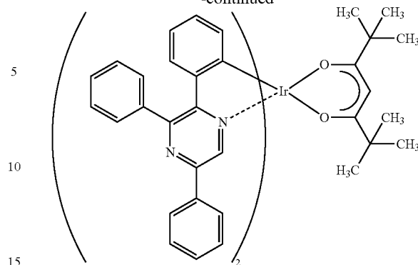
[Ir(tppr) 2 (dpm)]
