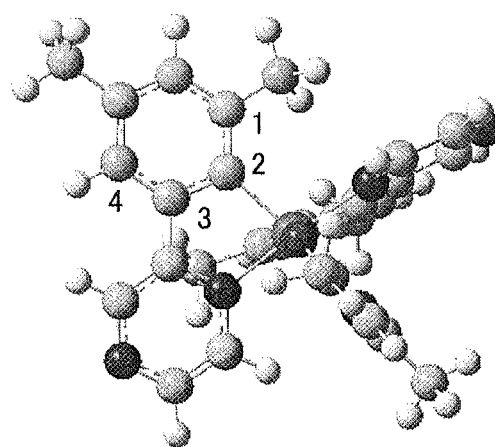
[\text{Ir}(\text{dmppr})_2(\text{acac})]
