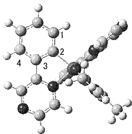
[\text{Ir}(\text{ppr})_2(\text{acac})]
