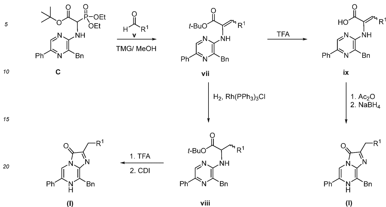
Scheme 3. Synthesis of the compound of formula (I)
