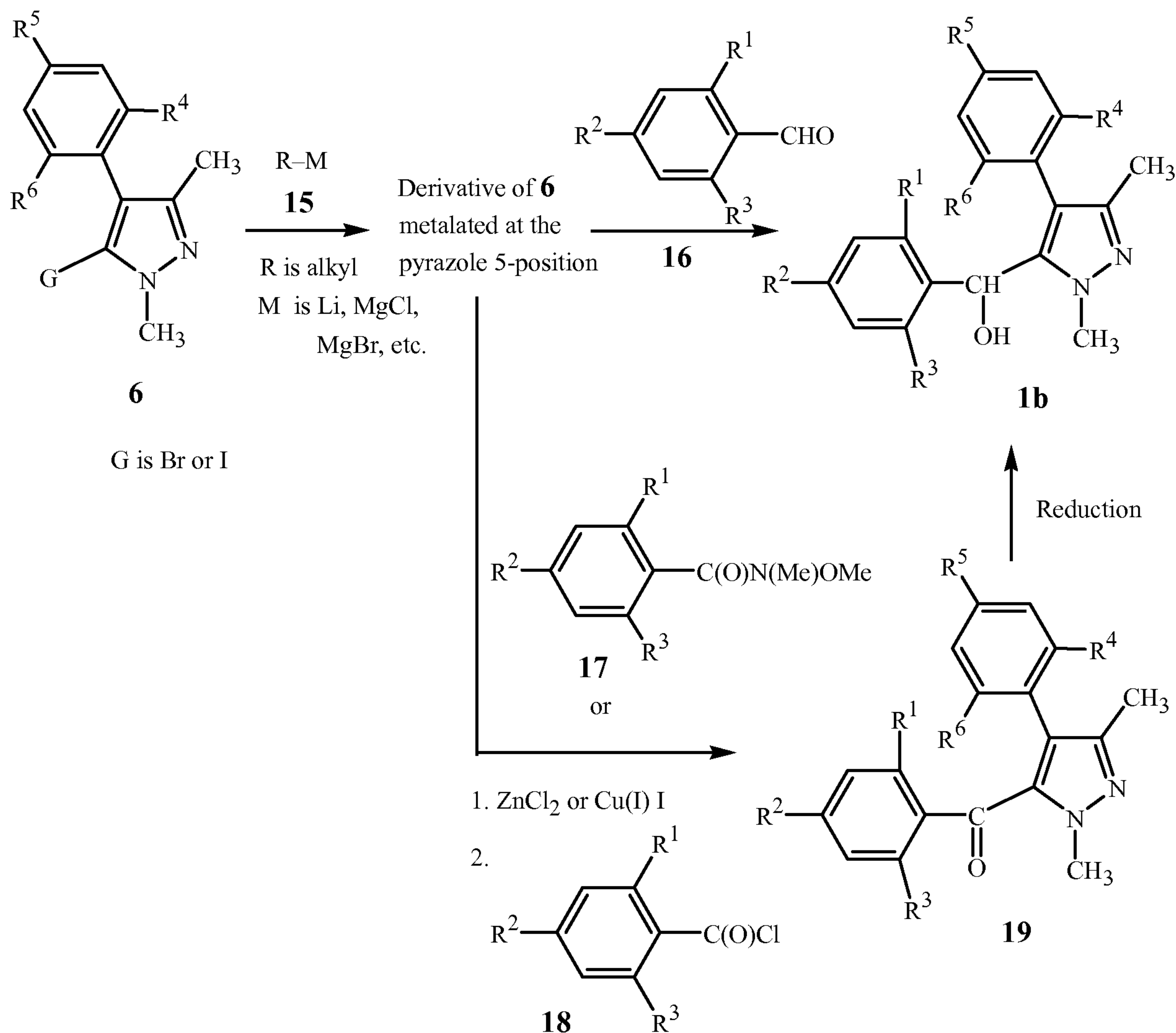
Scheme 12
