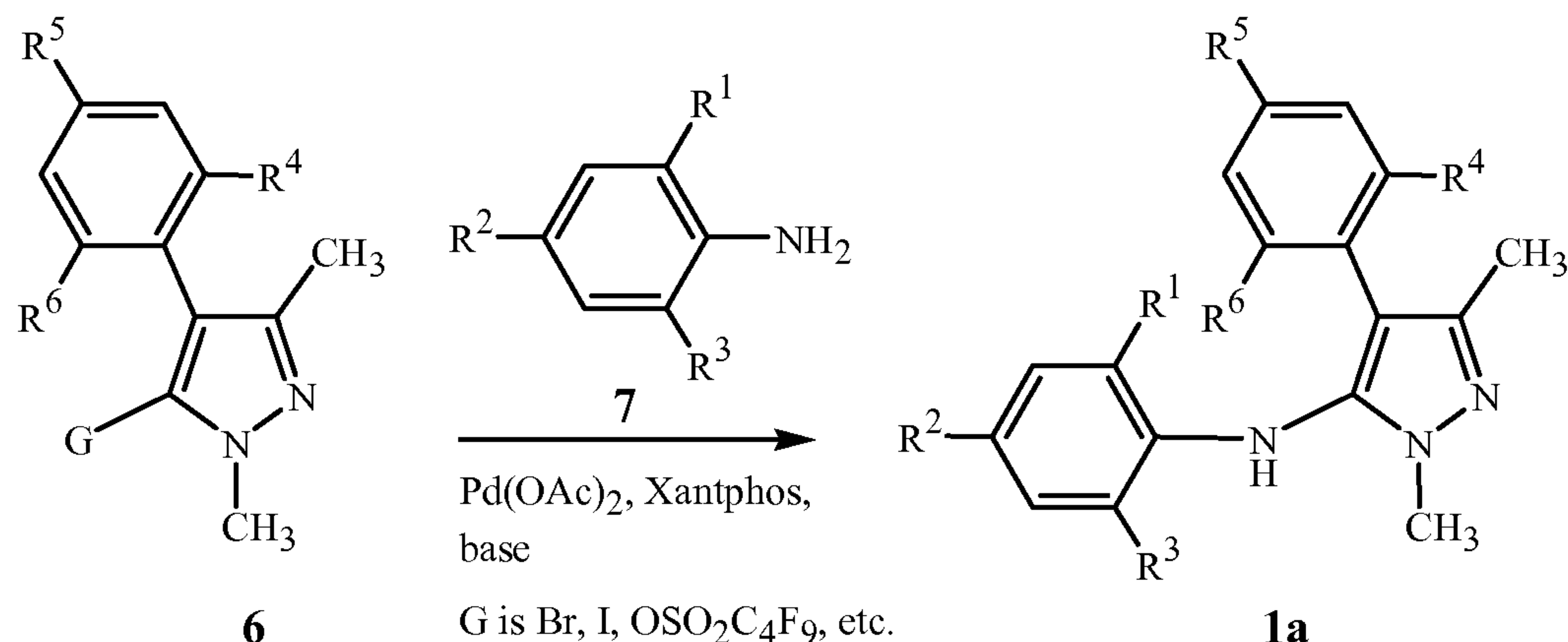
Scheme 3
