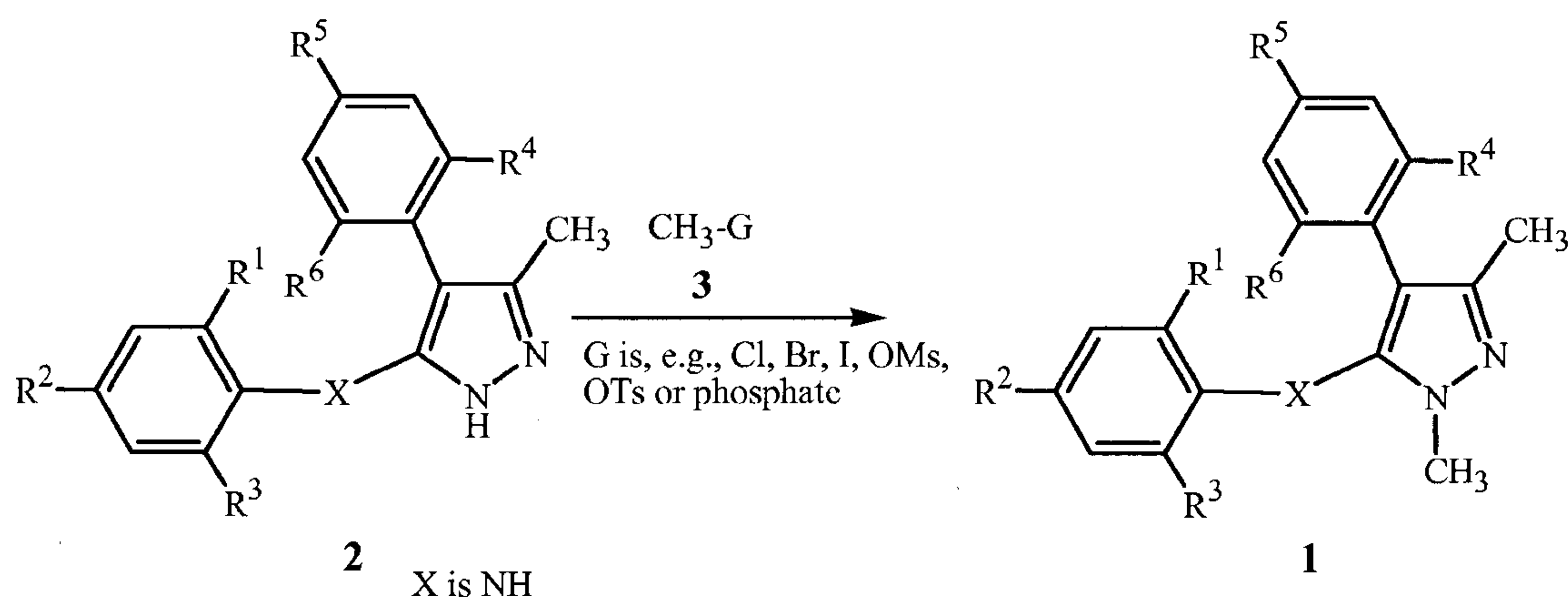
Scheme 1
