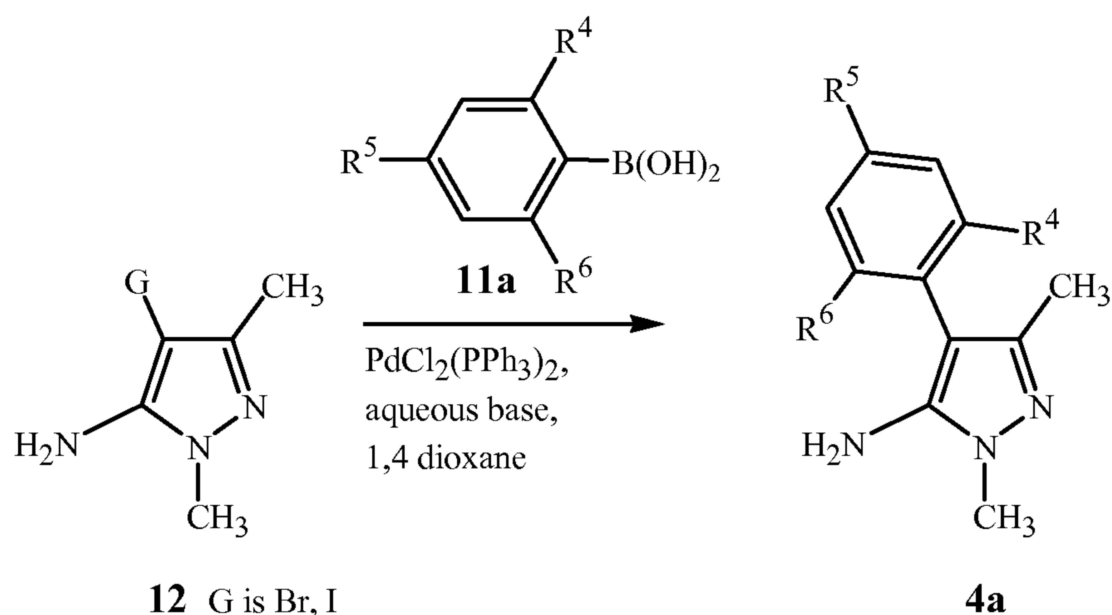
Scheme 8
