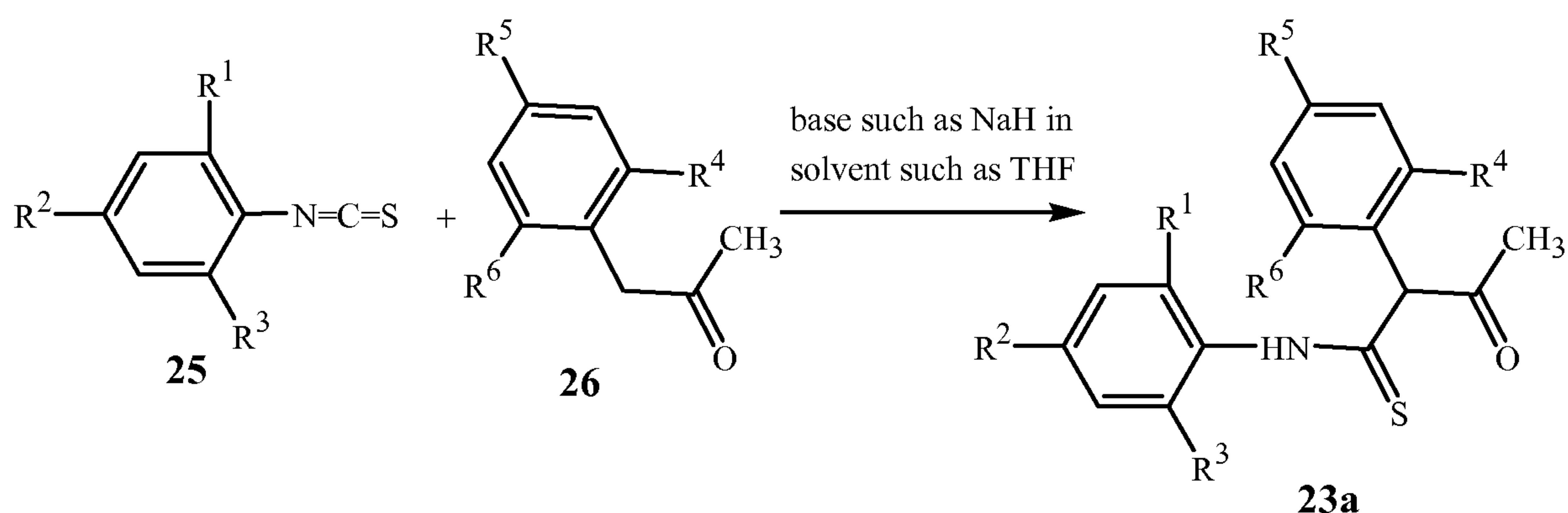
Scheme 17
