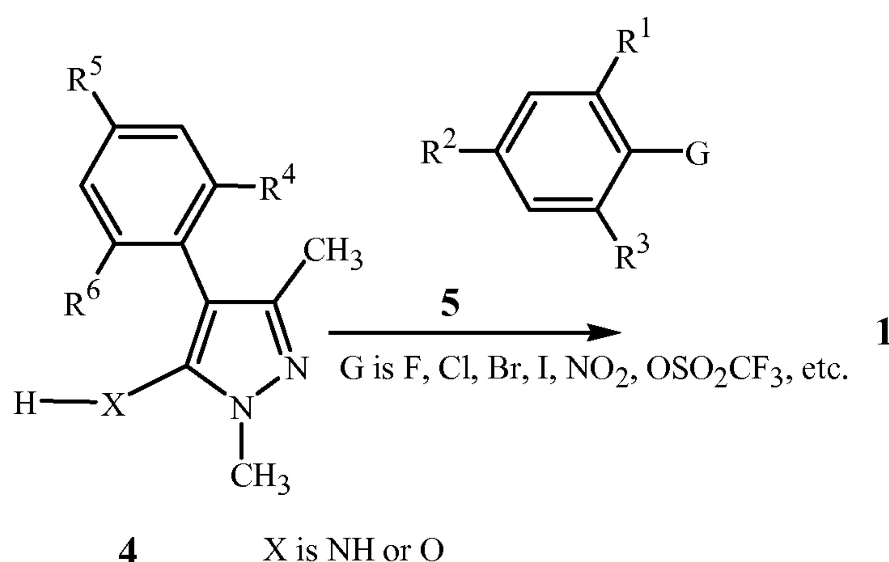
Scheme 2
