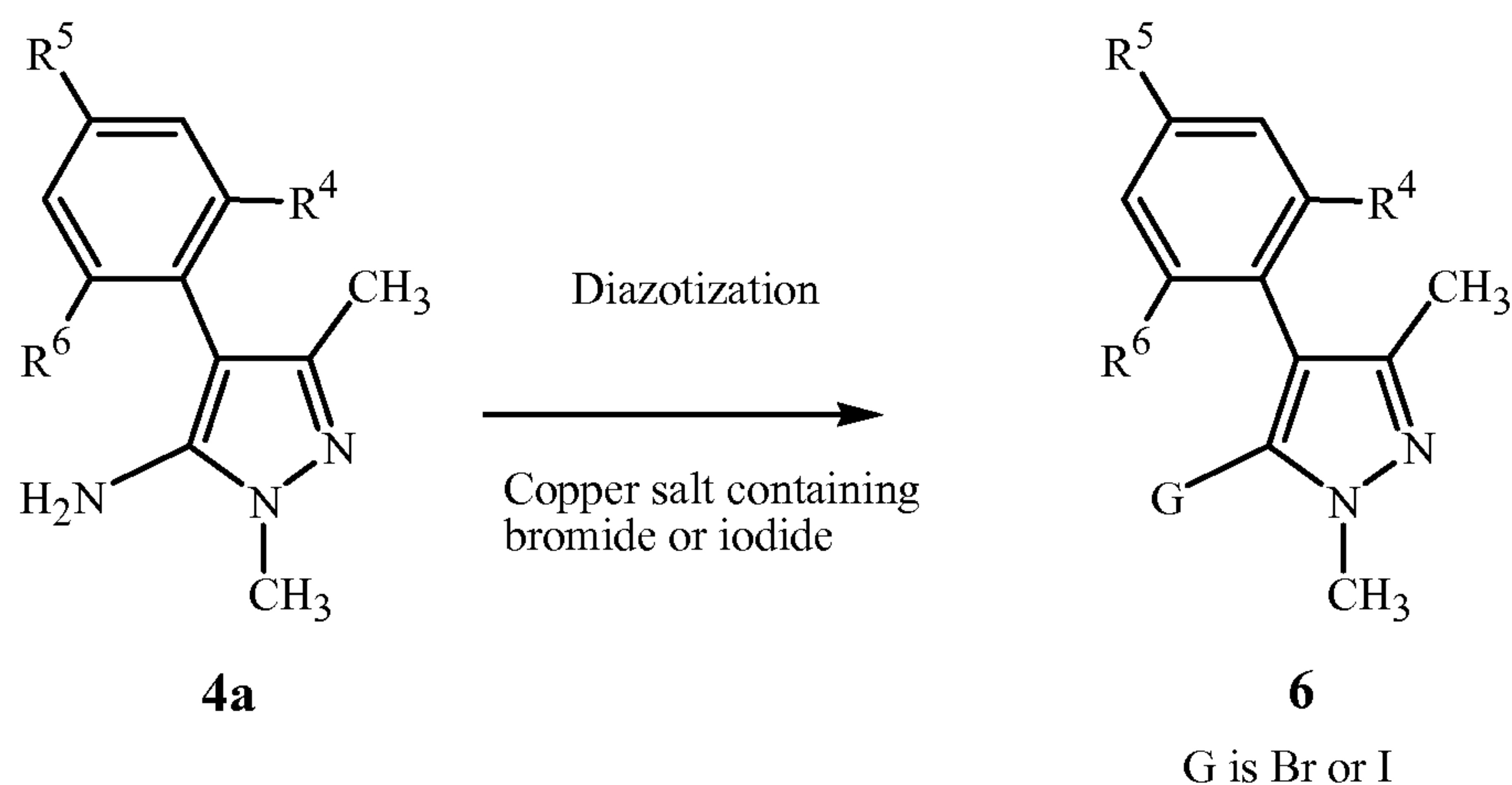
Scheme 4
