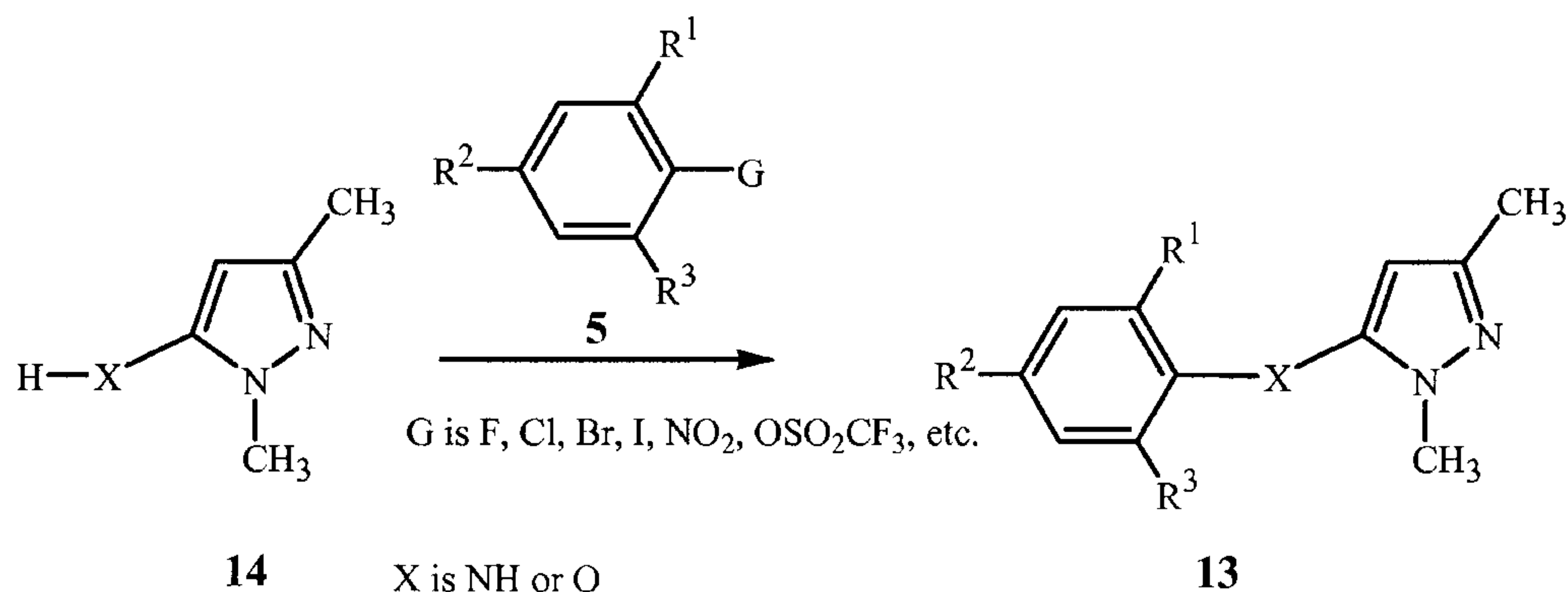
Scheme 11
