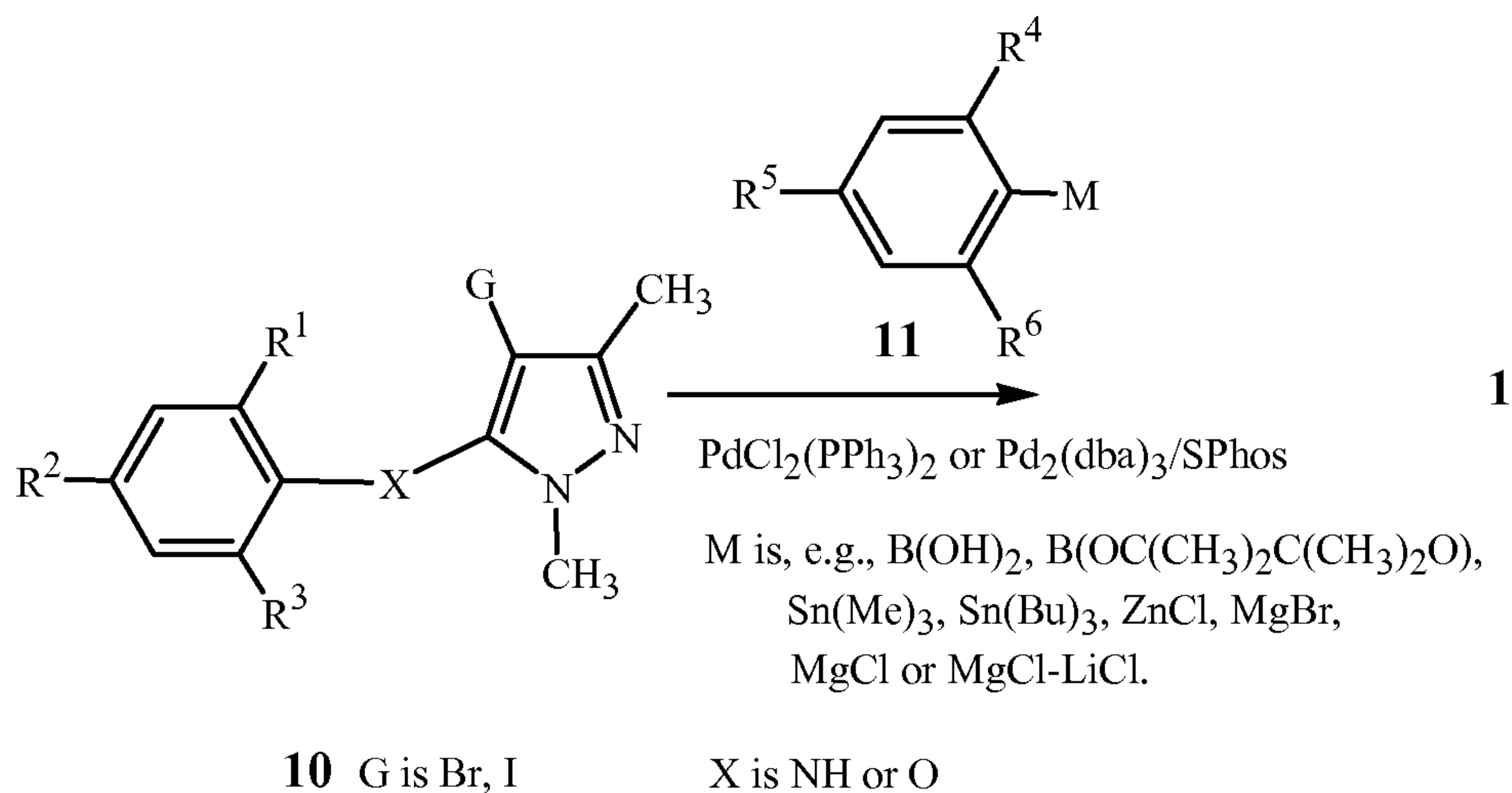
Scheme 7
