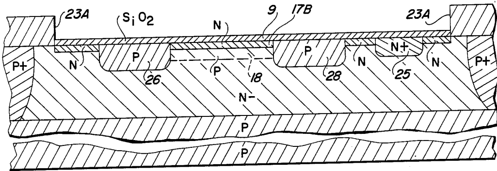
FIG. 1C PRIOR ART
