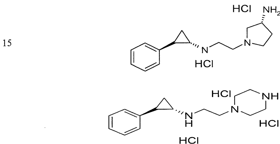
Compound 1(A)
