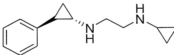
Compound 2(B)
