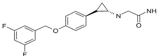
Compound 2(B)
