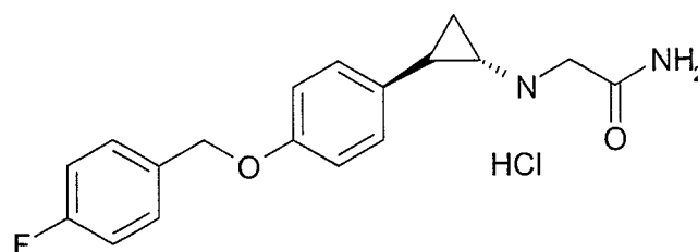
Compound 2(C)
